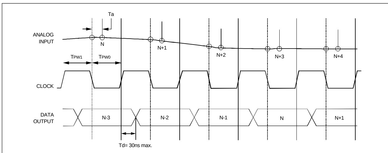
Figure 2. Timing Diagram
