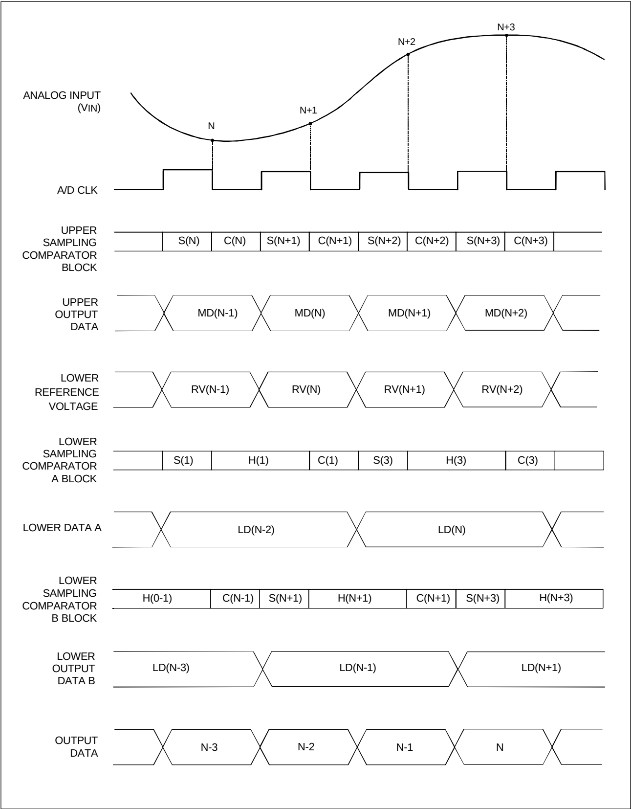
Figure 4. Timing Chart
