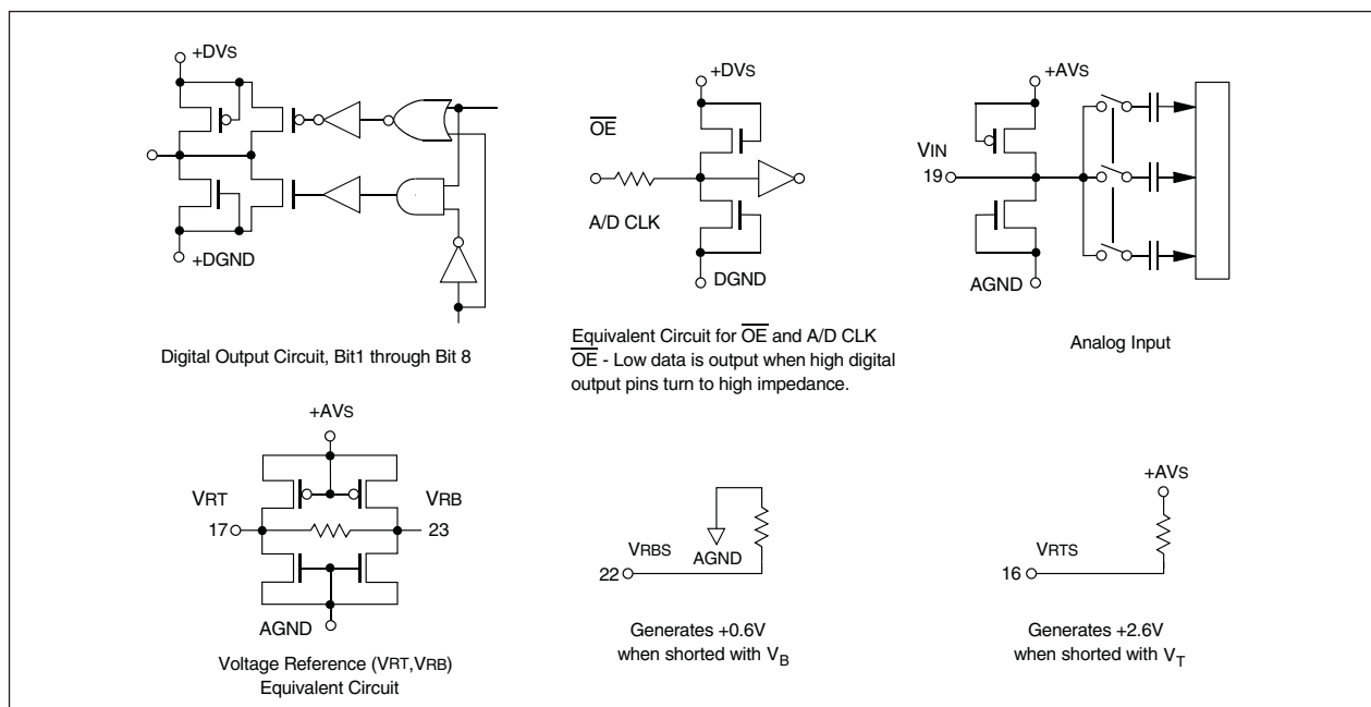
Figure 3. Equivalent Circuits
