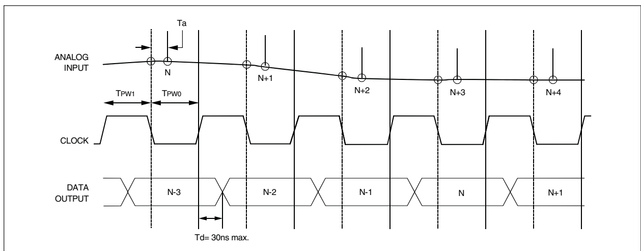
Figure 2. Timing Diagram
