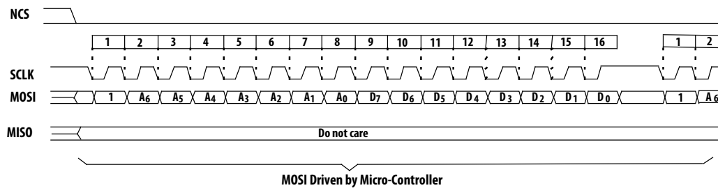
Figure 9. Write Operation
