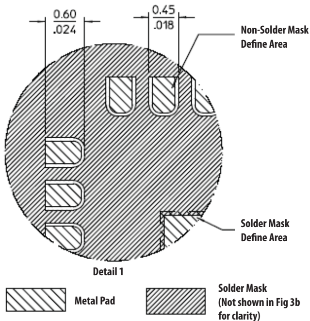
Figure 3c. Recommended Customer's PCB PADOUT and spacing
