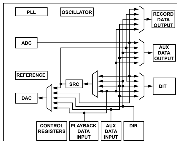
Figure 52. Datapath
