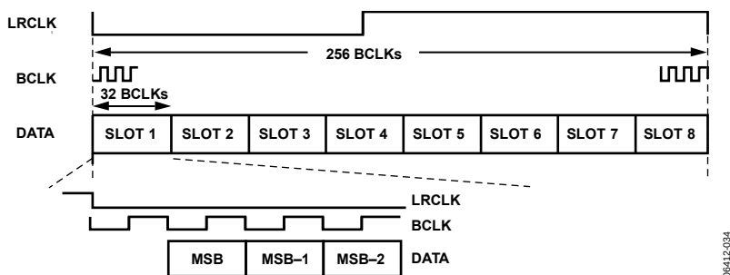
Figure 35. TDM Mode
