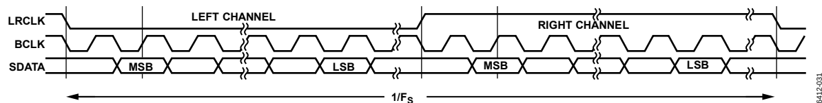
Figure 32. PS Mode—16 Bits to 24 Bits per Channel
