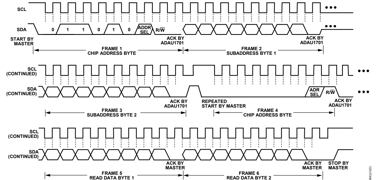
Figure 21. I 2 C Read from ADAU1701 Clocking
