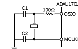
Figure 16. Crystal oscillator circuit
