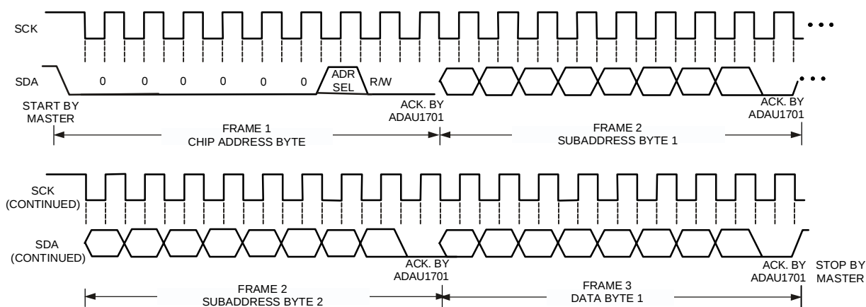
Figure 22. ADAU1701 I2C Write Clocking
