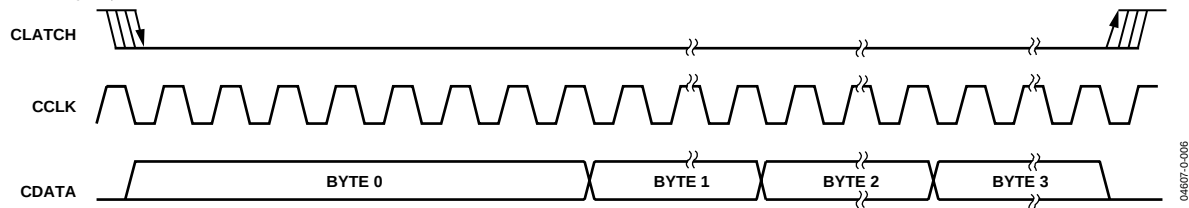
Figure 28. SPI Write Clocking (Single-Write Mode)
