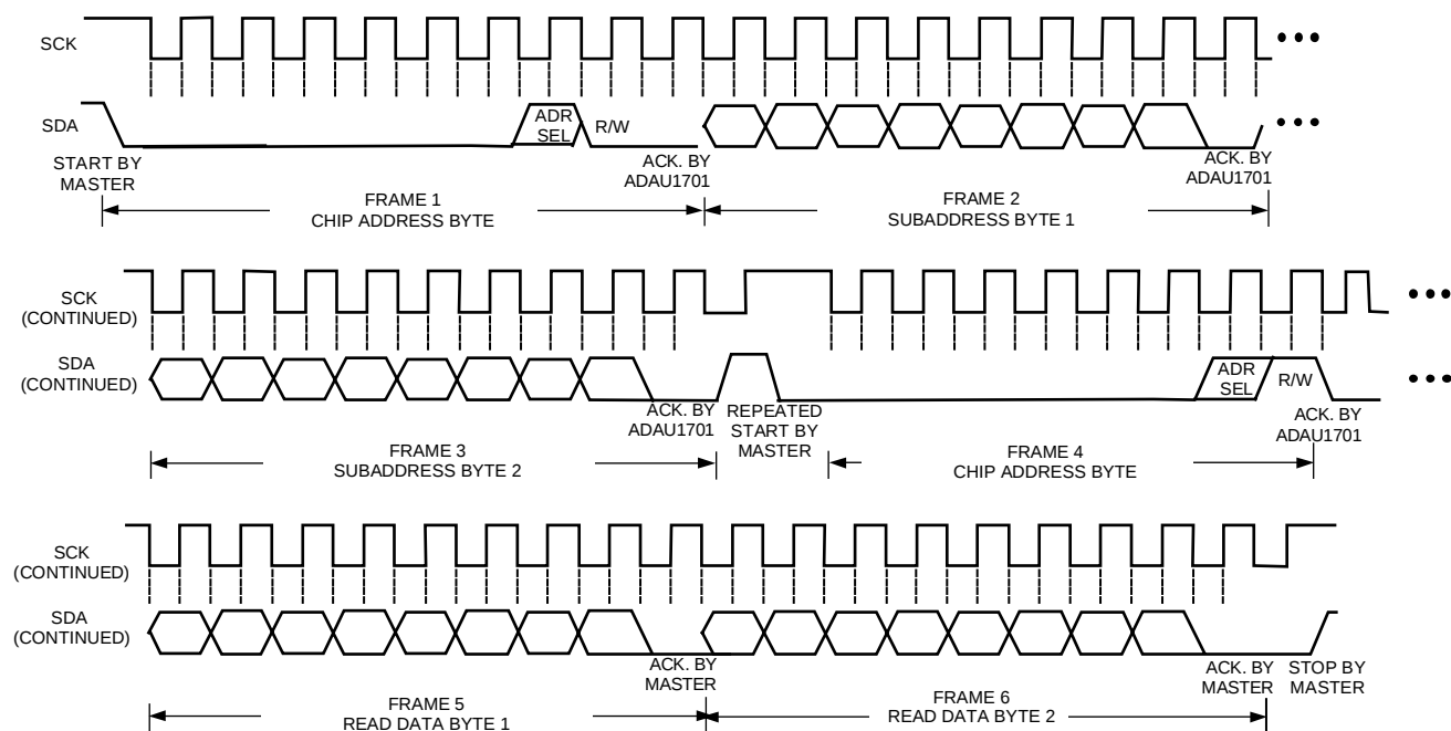
Figure 23. ADAU1701 I2C Read Clocking
