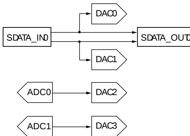
Figure 15. Default Program Signal Flow
