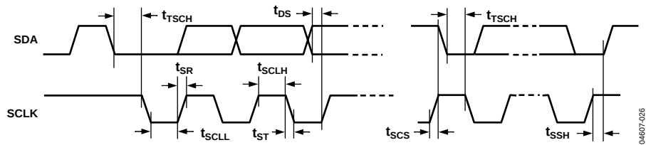
Figure 40. I²C Port Timing
