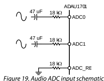
Figure 19. Audio ADC input schematic
