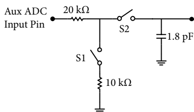
Figure 31. Auxiliary ADC input circuit
