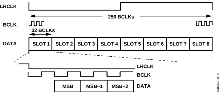
Figure 35. TDM Mode
