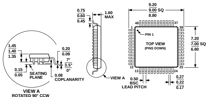
Figure 40. 48-Lead Low-Profile Quad Flat Package [LQFP] (ST-48)
