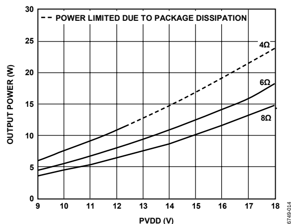
Figure 14. Output Power vs. PVDD @ 0.1% THD + N
