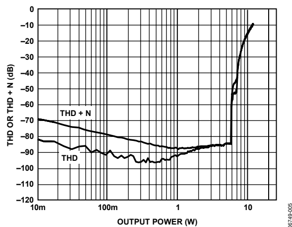
Figure 5. THD or THD + N vs. Output Power, 4 \Omega , PVDD = 9 V
