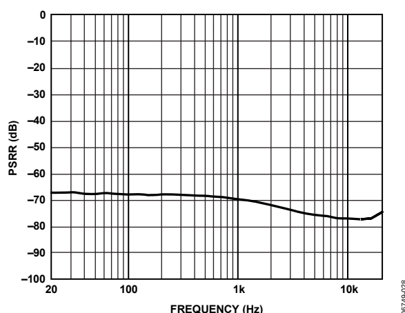
Figure 28. PSRR vs. Frequency, No Input Signal, Ripple = 1.5 V p-p, PVDD = 15 V, 6 Ω
