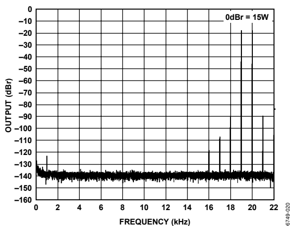
Figure 20. FFT @ 1 W, 6 \Omega , PVDD = 15 V, PGA = 0 dB, 19 kHz and 20 kHz Sine
