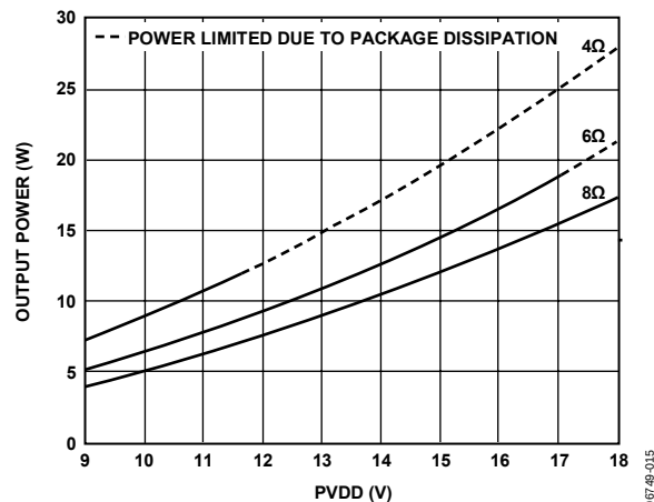
Figure 15. Output Power vs. PVDD @ 1% THD + N
