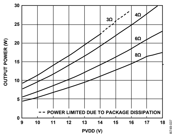
Figure 37. Output Power vs. PVDD, Mono Mode, 40 dB THD + N
