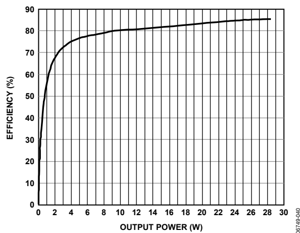
Figure 40. Efficiency vs. Output Power, Mono Mode, 15 V, 4 Ω
