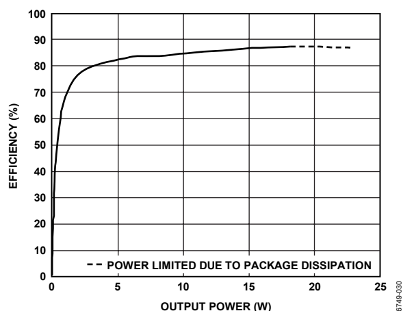
Figure 30. Efficiency vs. Output Power, 15 V, 6 \Omega
