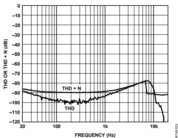
Figure 24. THD or THD + N vs. Frequency @ 1 W, 6 Ω, PVDD = 15 V, PGA = 0 dB
