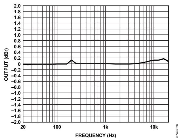
Figure 26. Frequency Response @ 1 W, 6 Ω, PVDD = 15 V, PGA = 0 dB
