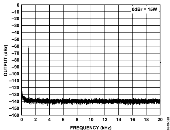
Figure 18. FFT @ -60 dBFS, 6 \Omega , PVDD = 15 V, PGA = 0 dB, 1 kHz Sine
