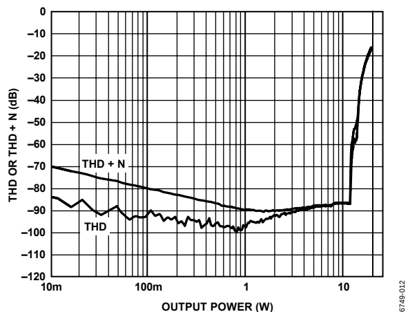
Figure 12. THD or THD + N vs. Output Power, 6 Ω, PVDD = 15 V
