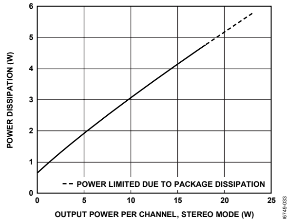
Figure 33. Power Dissipation vs. Output Power, 15 V, 6 \Omega , Stereo Mode, Both Channels Driven
