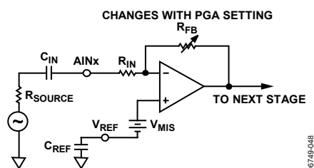
Figure 48. Input Equivalent Circuit
