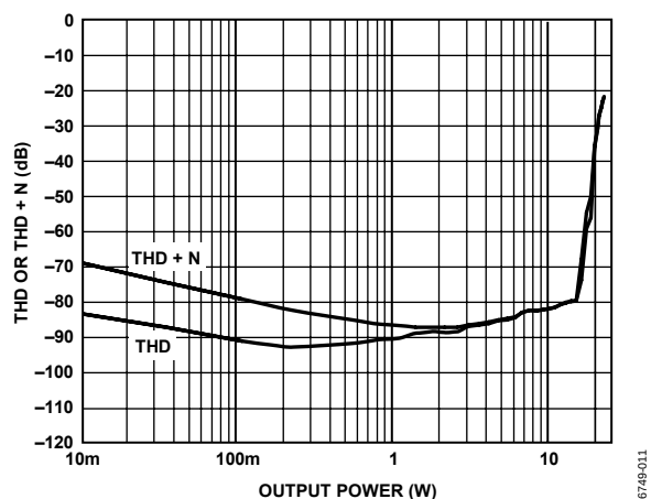
Figure 11. THD or THD + N vs. Output Power, 4 Ω, PVDD = 15 V
