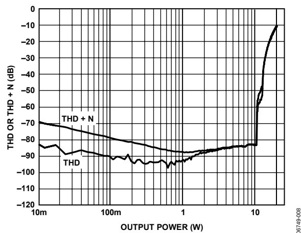
Figure 8. THD or THD + N vs. Output Power, 4 \Omega , PVDD = 12 V
