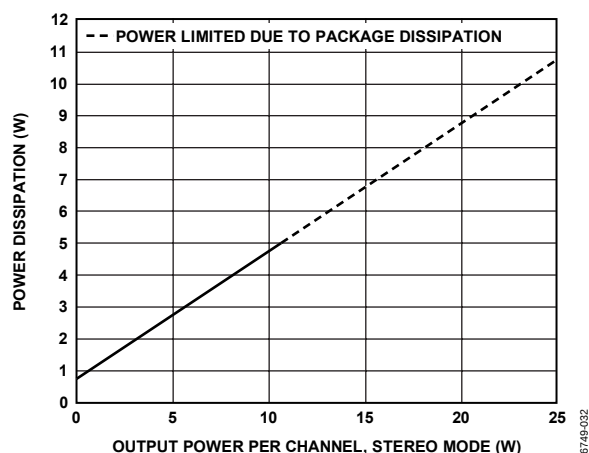
Figure 32. Power Dissipation vs. Output Power, 15 V, 4 \Omega , Stereo Mode, Both Channels Driven
