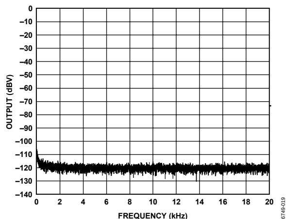
Figure 19. FFT No Input, 6 \Omega , PVDD = 15 V, PGA = 0 dB
