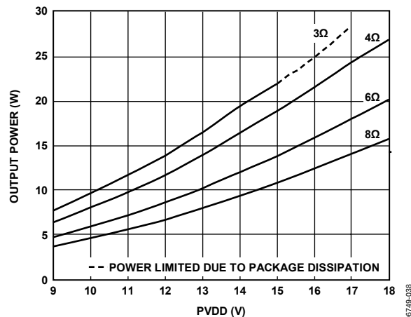
Figure 38. Output Power vs. PVDD, Mono Mode, 60 dB THD + N
