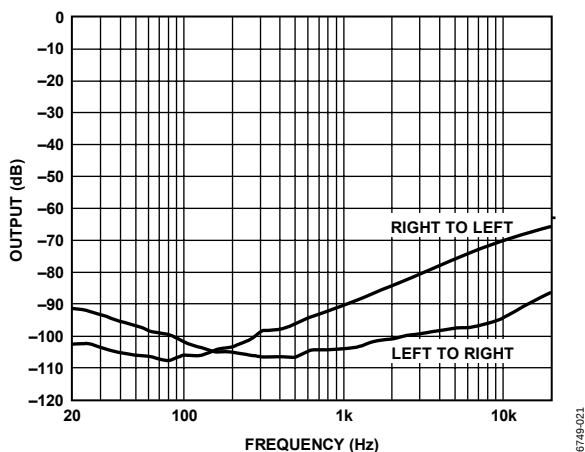
Figure 21. Crosstalk @ 1 W, 6 \Omega , PVDD = 15 V, PGA = 0 dB
