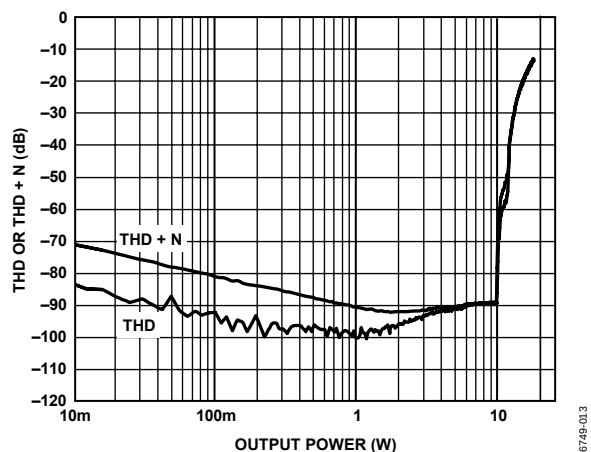
Figure 13. THD or THD + N vs. Output Power, 8 Ω, PVDD = 15 V
