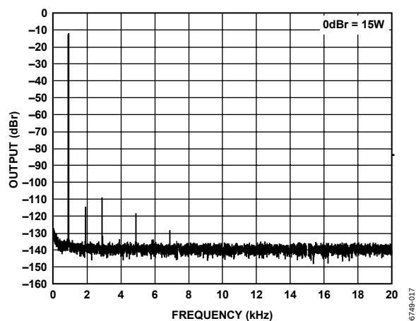
Figure 17. FFT @ 1 W, 6 \Omega , PVDD = 15 V, PGA = 0 dB, 1 kHz Sine
