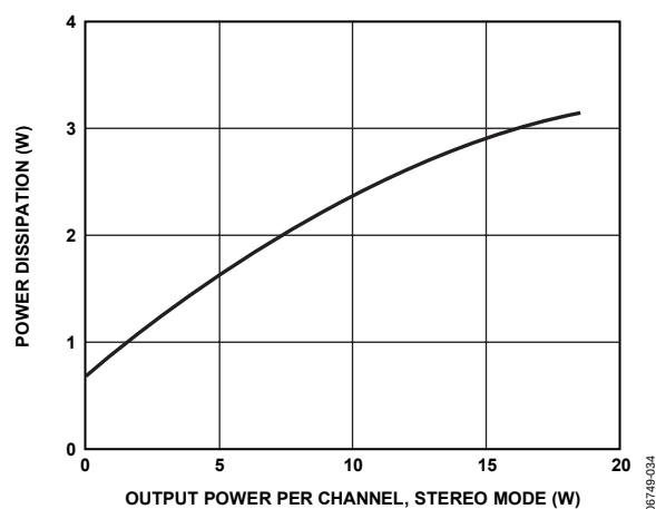
Figure 34. Power Dissipation vs. Output Power, 15 V, 8 \Omega , Stereo Mode, Both Channels Driven
