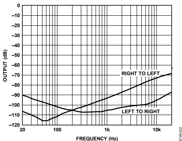
Figure 22. Crosstalk @ Full Scale, 6 \Omega , PVDD = 15 V, PGA = 0 dB
