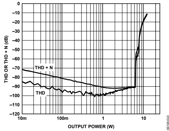
Figure 10. THD or THD + N vs. Output Power, 8 \Omega , PVDD = 12 V
