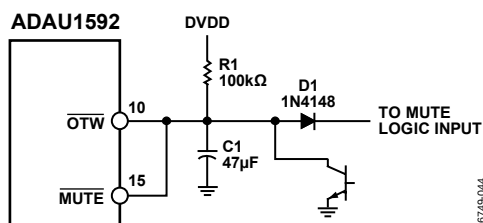
Figure 44. Option 1 Schematic for Autorecovery
