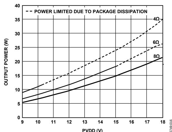
Figure 16. Output Power vs. PVDD @ 10% THD + N
