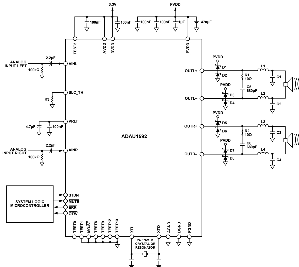
Figure 49. Typical Stereo Application Circuit
