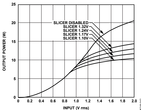
Figure 42. Typical Output Power vs. Input at Different Slicer Settings
