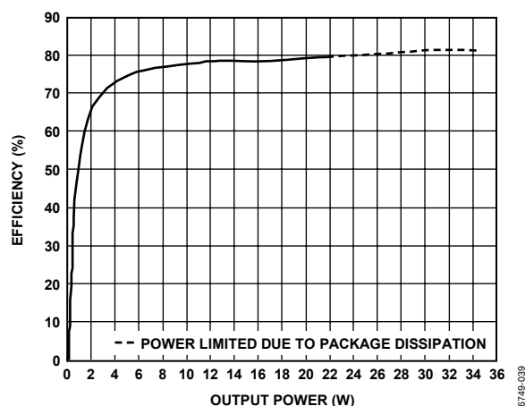
Figure 39. Efficiency vs. Output Power, Mono Mode, 15 V, 3 Ω
