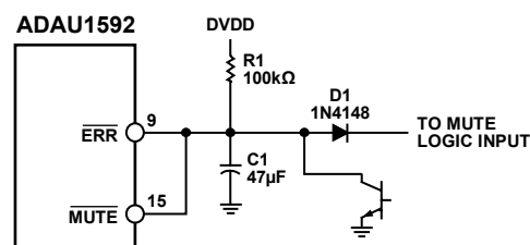
Figure 45. Option 2 Schematic for Autorecovery
