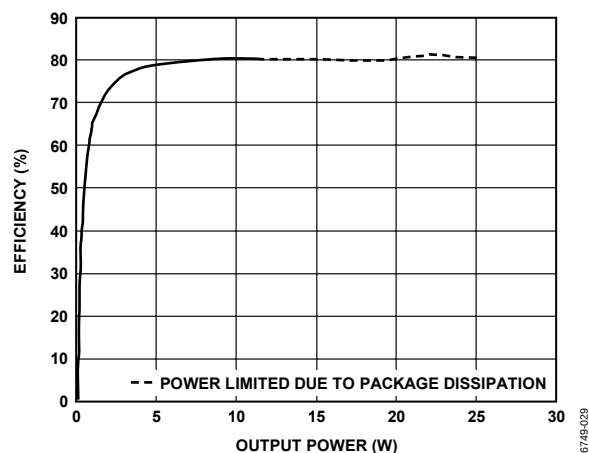
Figure 29. Efficiency vs. Output Power, 15 V, 4 \Omega
