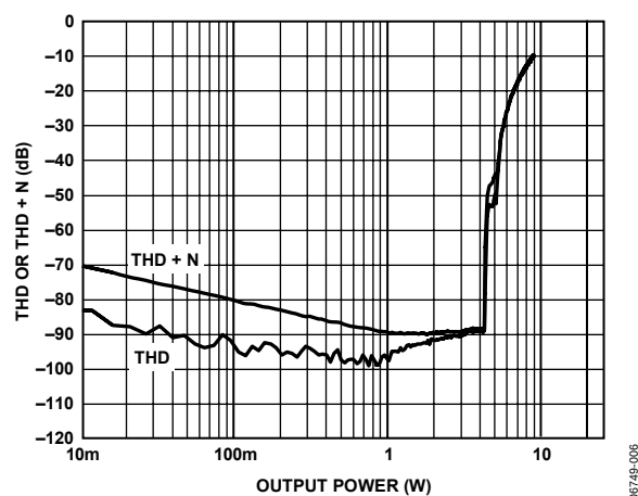
Figure 6. THD or THD + N vs. Output Power, 6 \Omega , PVDD = 9 V
