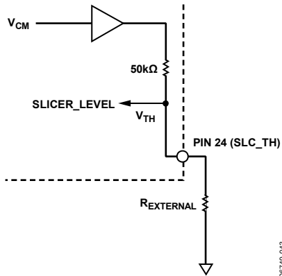
Figure 43. Block for Slicer Threshold Adjust, SLC_TH
