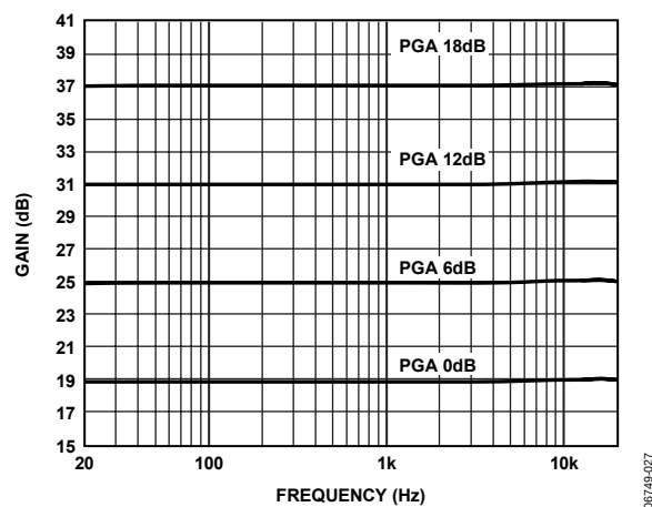
Figure 27. Gain vs. Frequency @ 1 W, 6 Ω, PVDD = 15 V
