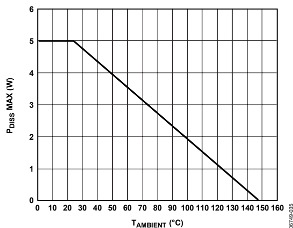
Figure 35. Power Dissipation Derating vs. Ambient Temperature
