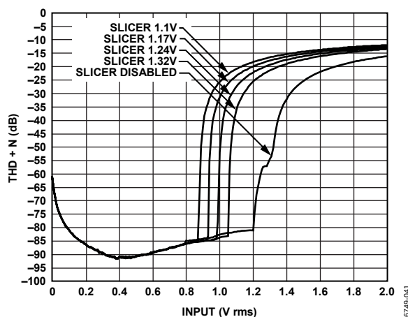
Figure 41. THD + N vs. Input Level @ PGA = 0 dB, 15 V
