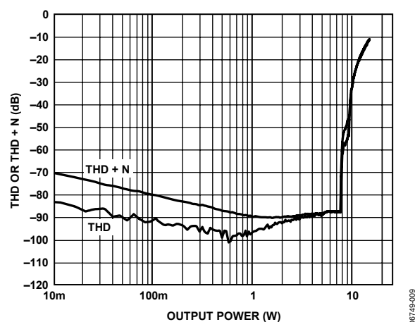
Figure 9. THD or THD + N vs. Output Power, 6 \Omega , PVDD = 12 V
