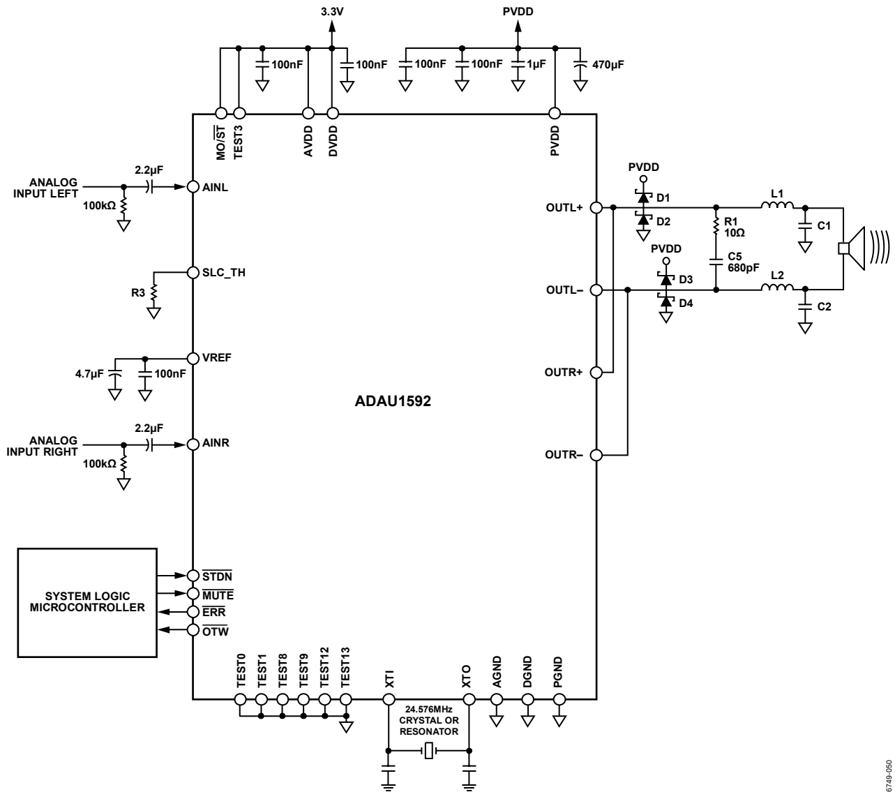
Figure 50. Typical Mono Application Circuit
