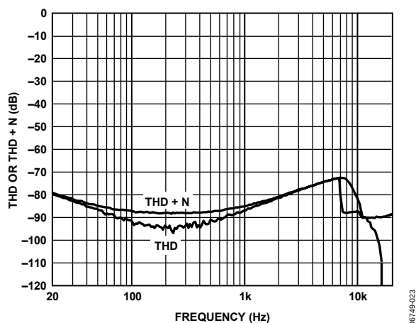
Figure 23. THD or THD + N vs. Frequency @ 1 W, 4 Ω, PVDD = 15 V, PGA = 0 dB
