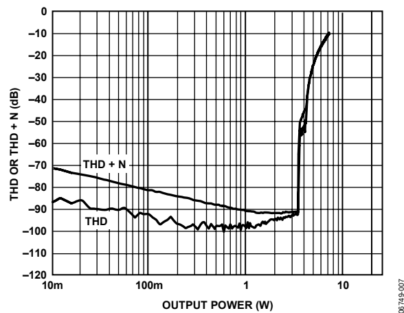
Figure 7. THD or THD + N vs. Output Power, 8 \Omega , PVDD = 9 V
