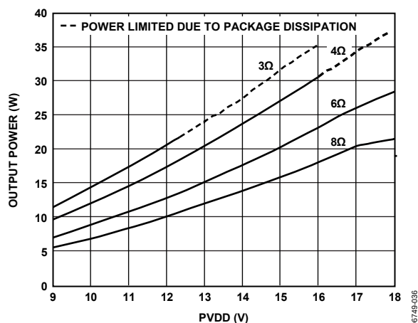
Figure 36. Output Power vs. PVDD, Mono Mode, 20 dB THD + N
