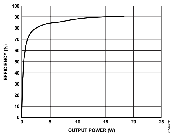
Figure 31. Efficiency vs. Output Power, 15 V, 8 \Omega
