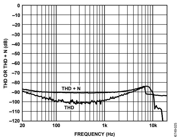
Figure 25. THD or THD + N vs. Frequency @ 1 W, 8 Ω, PVDD = 15 V, PGA = 0 dB
