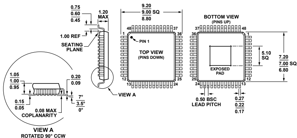
Figure 52. 48-Lead Thin Quad Flat Package, Exposed Pad [TQFP_EP]
