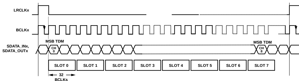
Figure 26. TDM Mode with Pulse Frame Clock
