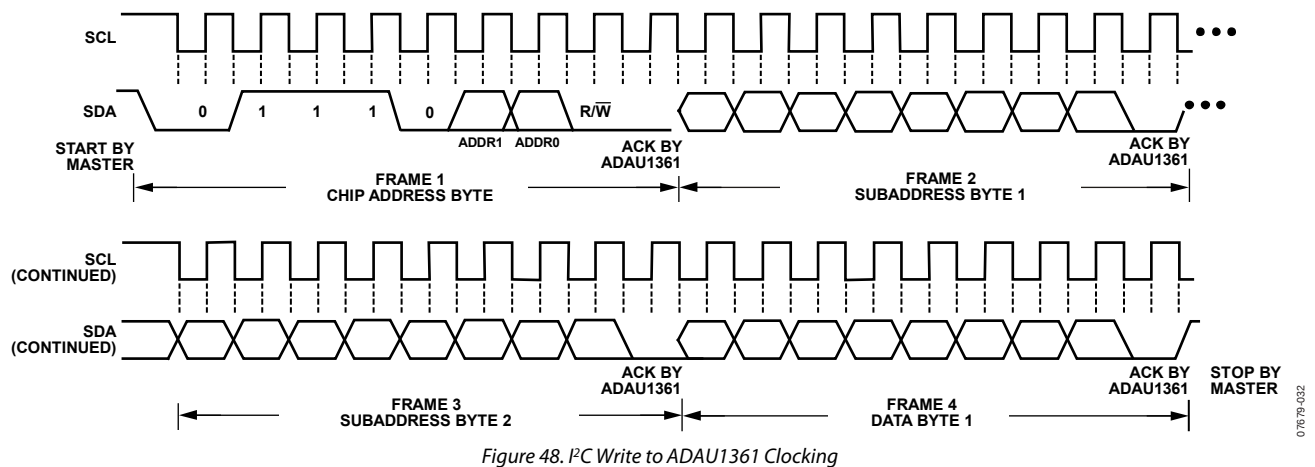
Figure 48. I 2 C Write to ADAU1361 Clcking
