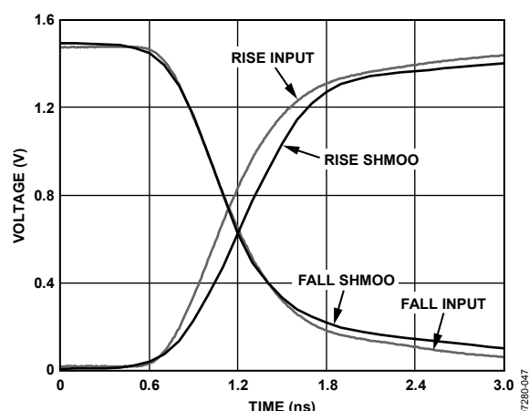
Figure 32. Comparator Shmoo, 1.5\text{ V} Input, 1.2\text{ ns} (10% to 90%) Input, 50\ \Omega Terminated
