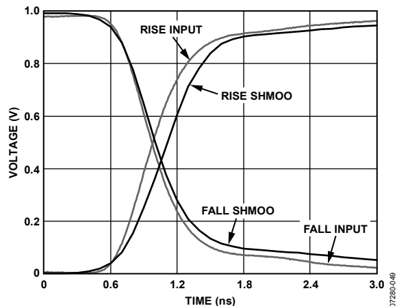
Figure 30. Comparator Shmoo, 1.0\text{ V} Input, 1.0\text{ ns} (10% to 90%) Input, 50\ \Omega Terminated
