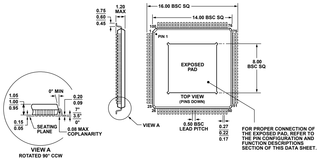
Figure 85. 100-Lead, Thin Quad Flatpack, Exposed Pad [TQFP_EP] (SV-100-7)
