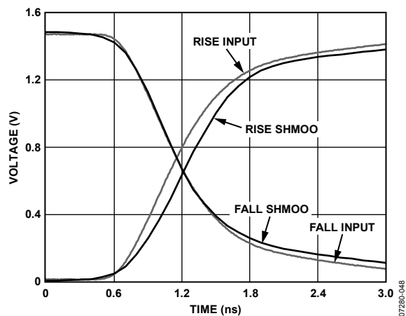
Figure 31. Comparator Shmoo, 1.5\text{ V} Input, 1.5\text{ ns} (10% to 90%) Input, 50\ \Omega Terminated
