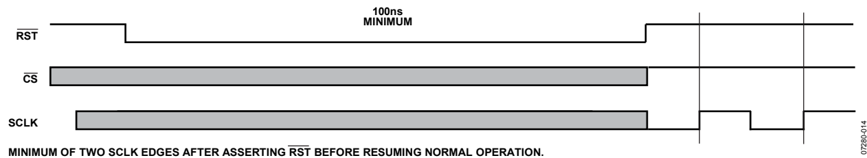
Figure 78. Reset Operation
