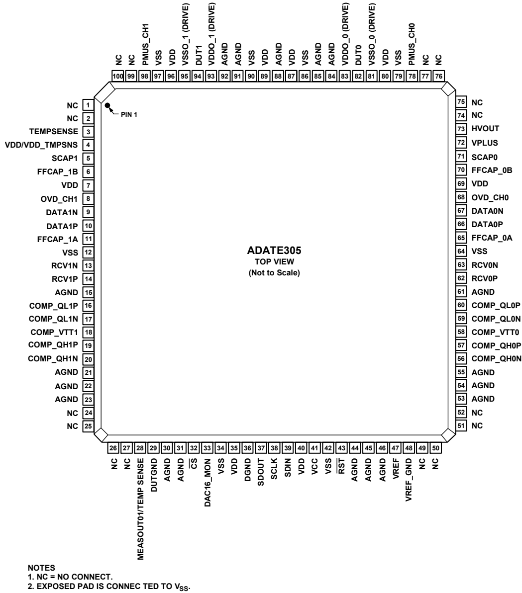
Figure 2. Pin Configuration
