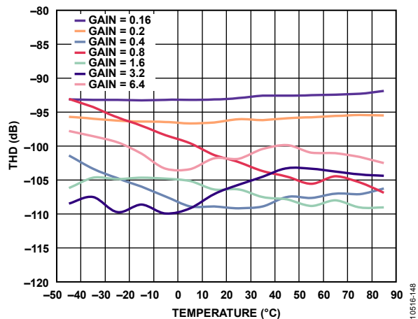
Figure 45. THD vs. Temperature
