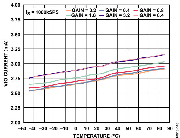
Figure 43. VIO Current vs. Temperature
