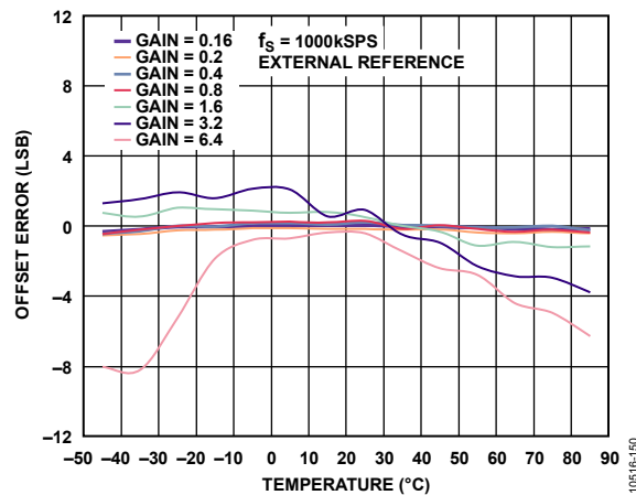
Figure 47. Offset Error vs. Temperature
