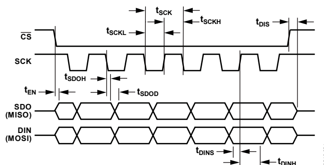
Figure 69. Serial Timing
