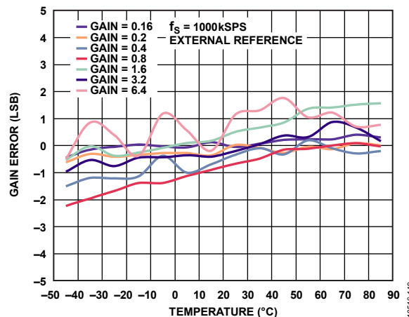
Figure 46. Gain Error vs. Temperature
