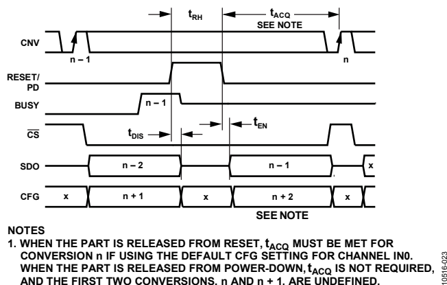
Figure 68. RESET and PD Timing
