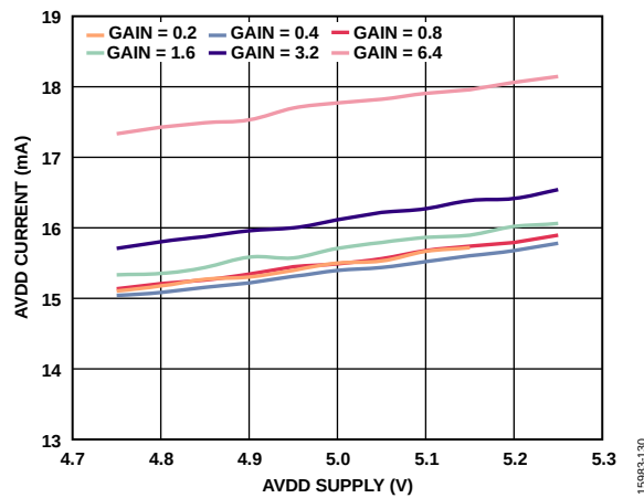
Figure 31. AVDD Current vs. AVDD Supply, Internal Reference
