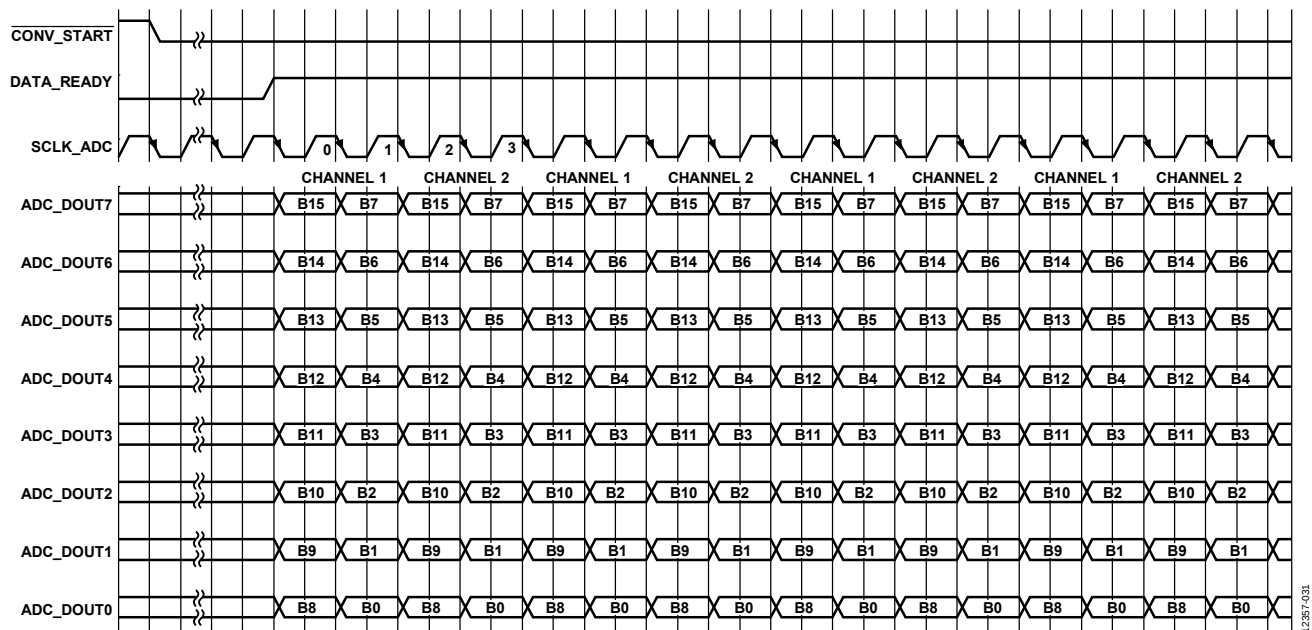
Figure 45. PPI, 2-Channel
