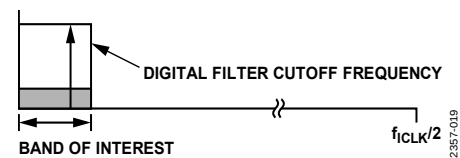
Figure 27. \Sigma - \Delta ADC, Digital Filter Cutoff Frequency
