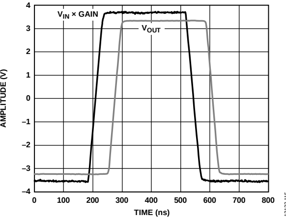
Figure 14. Overdrive Recovery
