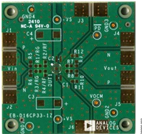
Figure 1. Component Side (LFCSP)
