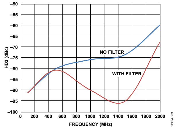
Figure 48. HD3 vs. Frequency, with and Without LC Filter
