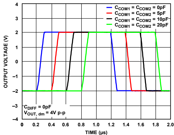
Figure 91. Large Signal Transient Response for Various Capacitive Loads, V_S = 3 \text{ V}
