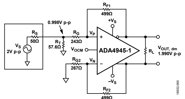
Figure 109. Terminated Single-Ended-to-Differential System with G = 1
