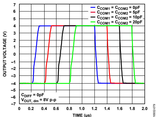
Figure 90. Large Signal Transient Response for Various Capacitive Loads, V_S = 5V
