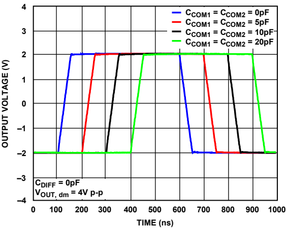
Figure 46. Large Signal Transient Response for Various Capacitive Loads, V_S = 3\text{ V}
