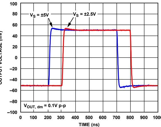
Figure 47. V_{OCM} Small Signal Transient Response
