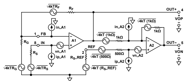
Figure 53. Noise Sources
