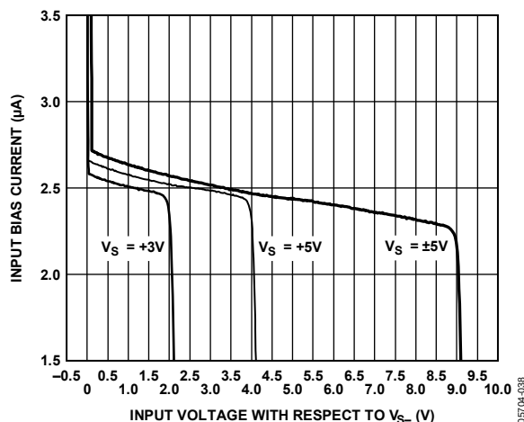
Figure 40. Input Bias Current vs. Input Voltage
