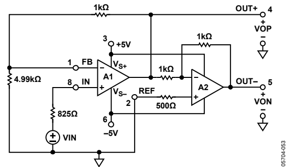
Figure 49. Dual Supply, G = 2.4, Single-Ended-to-Differential Amplifier
