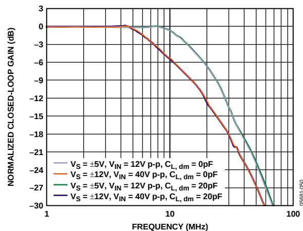
Figure 14. Large Signal Frequency Response for Various Capacitive Loads
