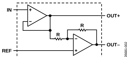
Figure 41. Functional Diagram
