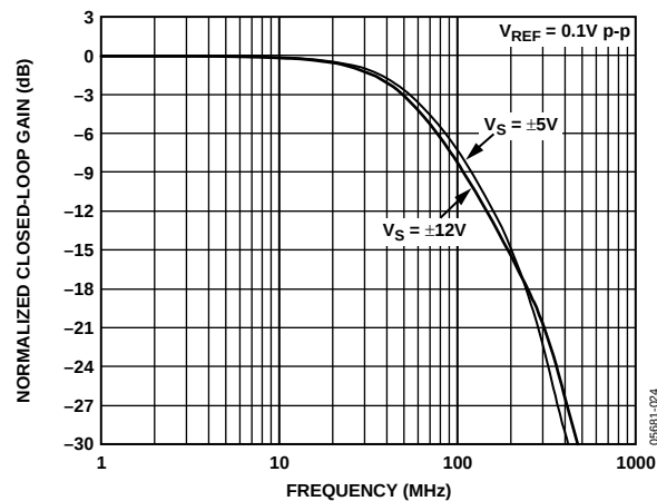
Figure 16. REF Small Signal Frequency Response for Various Power Supplies
