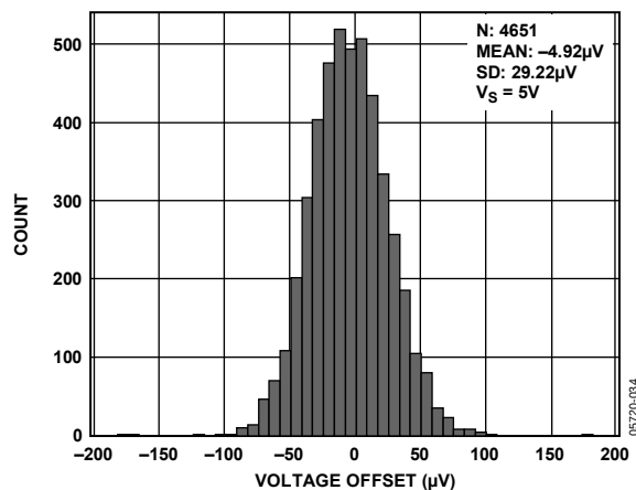
Figure 38. Input Offset Voltage Distribution ( V_S = 5\text{ V} )
