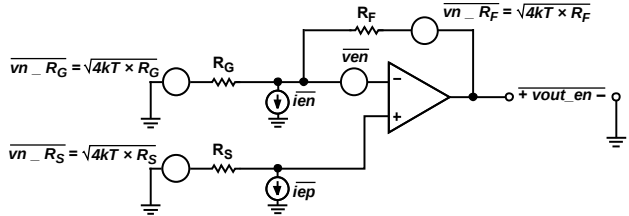
Figure 48. Noise Sources in Typical Connection
