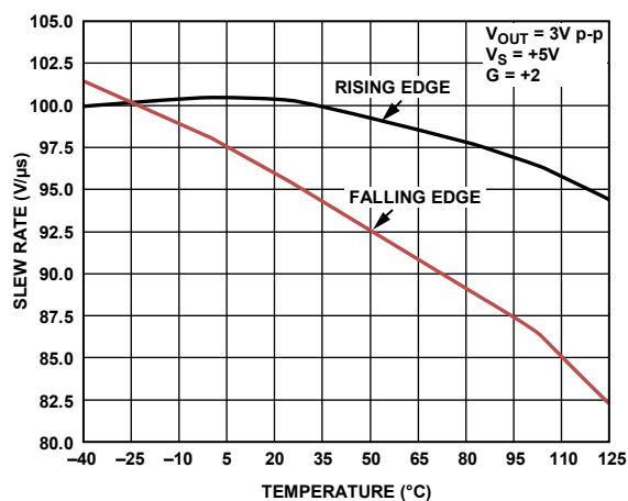
Figure 32. Slew Rate vs. Temperature
