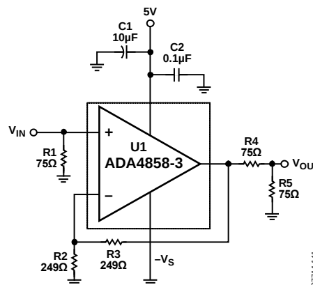
Figure 40. DC-Coupled, Single-Supply Schematic
