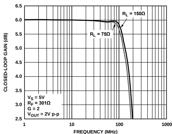
Figure 42. Large Signal Frequency Response for Various Loads
