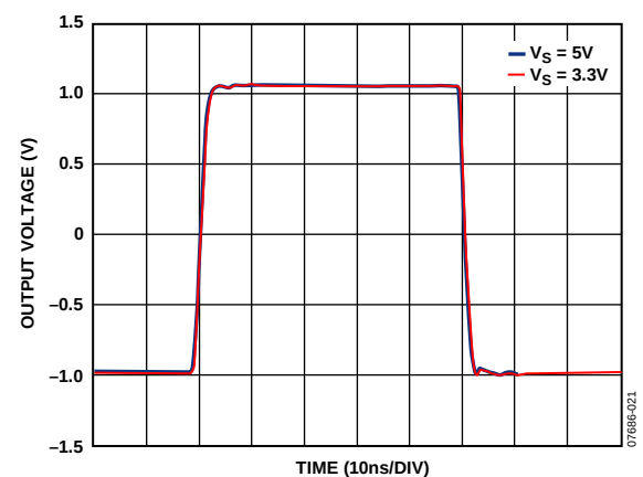
Figure 21. Large Signal Transient Response vs. Supply Voltage
