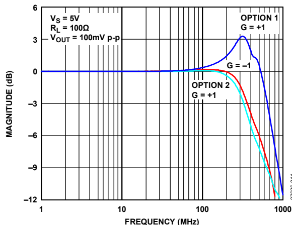
Figure 37. G = +1 and G = -1
