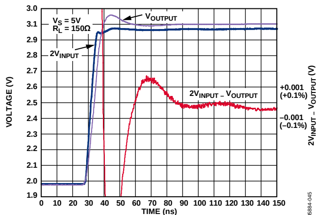
Figure 46. 0.1% Settling Time
