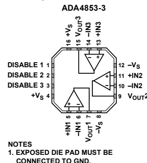
Figure 3. 16-Lead LFCSP_WQ
