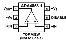
Figure 1. 6-Lead SC70
