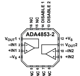
Figure 2. 16-Lead LFCSP_WQ
