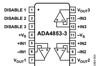
Figure 4. 14-Lead TSSOP
