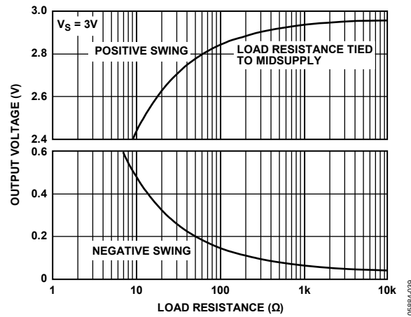
Figure 41. Output Voltage vs. Load Resistance
