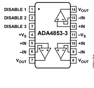
Figure 4. 14-Lead TSSOP
