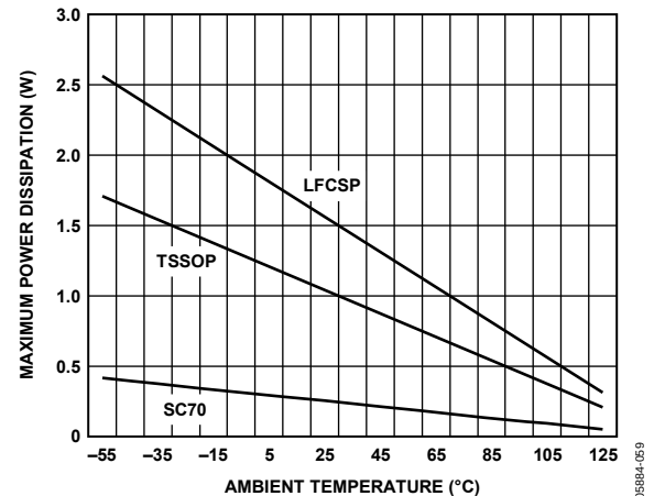
Figure 6. Maximum Power Dissipation vs. Temperature for a 4-Layer Board
