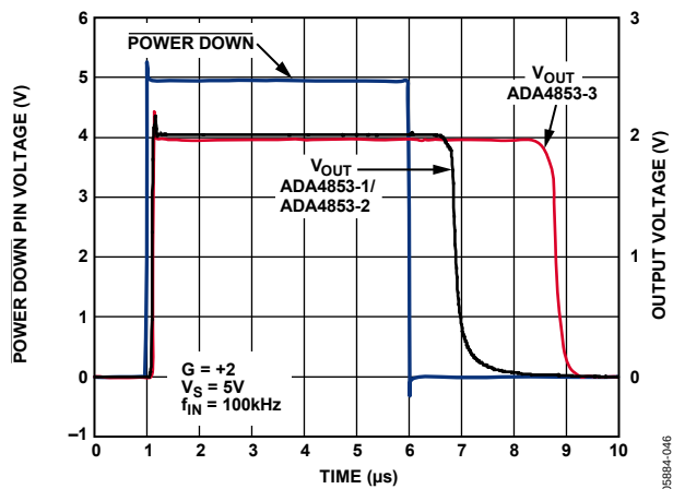
Figure 47. Enable/Disable Time
