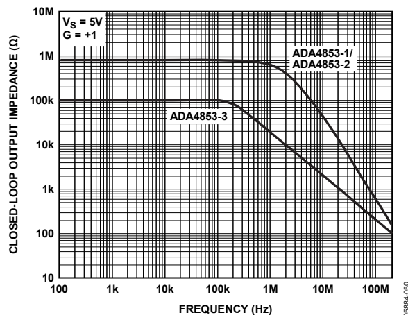
Figure 22. Output Impedance vs. Frequency Disabled
