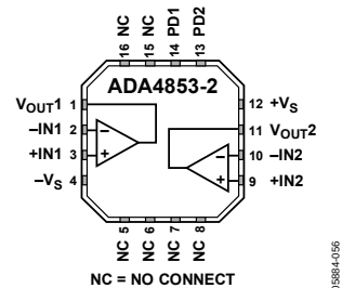
Figure 2. 16-Lead LFCSP_VQ
