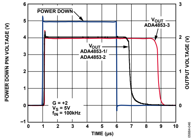
Figure 47. Enable/Disable Time
