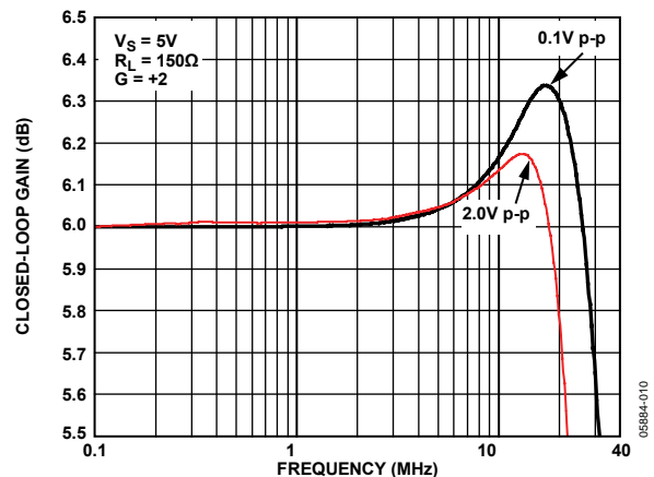
Figure 5. 0.5 dB Flatness Frequency Response
