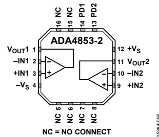
Figure 2. 16-Lead LFCSP_VQ
