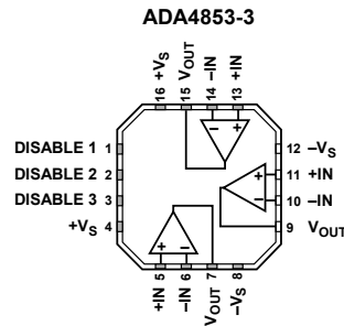
Figure 3. 16-Lead LFCSP_VQ
