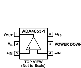
Figure 1. 6-Lead SC70
