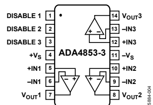
Figure 4. 14-Lead TSSOP
