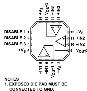
Figure 3. 16-Lead LFCSP_WQ
