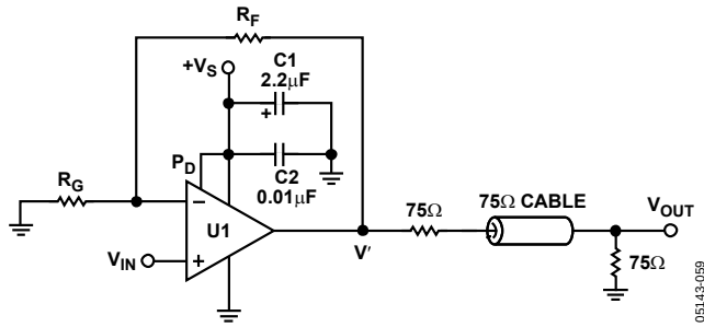
Figure 45. Video Amplifier
