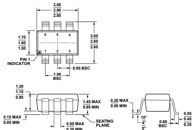
Figure 48. 6-Lead Small Outline Transistor Package [SOT-23] (RJ-6) Dimensions shown in millimeters
