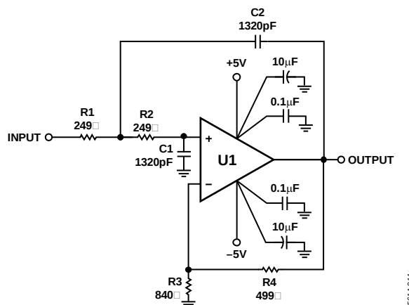
Figure 49. Two-Pole 500 kHz Reconstruction Filter Schematic
