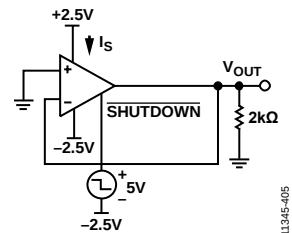
Figure 50. Turn-Off Response Test Circuit (See Figure 39 and Figure 41)
