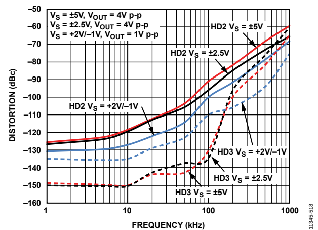
Figure 19. Distortion vs. Frequency, G = +2
