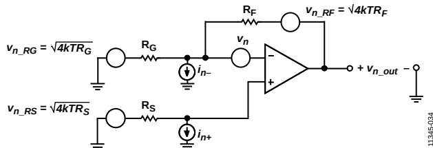
Figure 54. Noise Sources in Typical Connection
