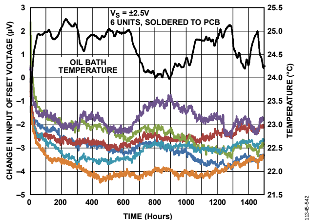
Figure 45. Long-Term V_{OS} Drift
