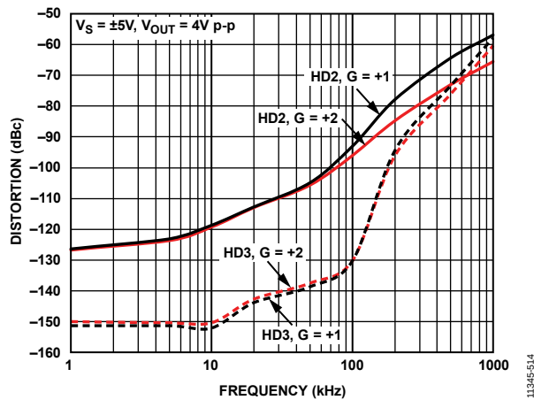
Figure 15. Distortion vs. Frequency for Various Gains
