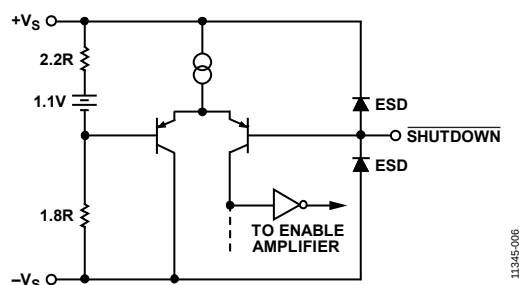
Figure 53. Shutdown Circuit
