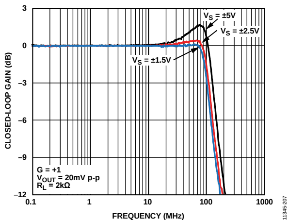
Figure 10. Small Signal Frequency Response for Various Supply Voltages
