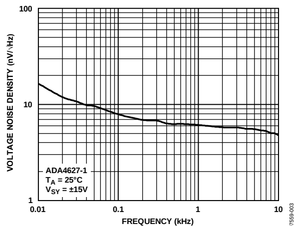
Figure 4. Voltage Noise Density vs. Frequency
