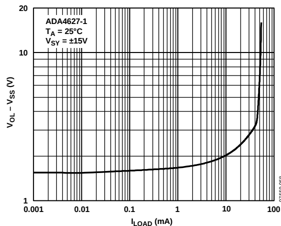
Figure 14. V_{OUT} Sinking vs. I_{LOAD} Current
