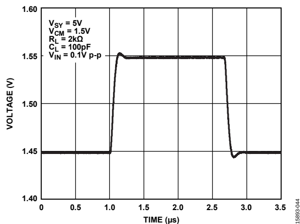
Figure 45. Small Signal Transient Response, A_V = -1 , V_{SY} = 5\text{ V}
