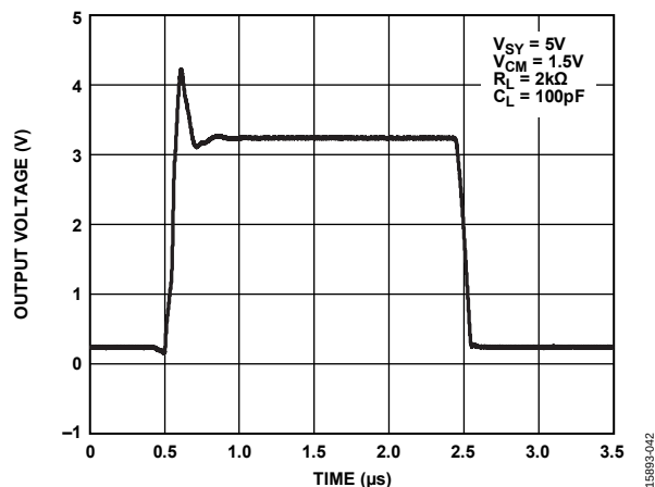
Figure 43. Large Signal Transient Response, A_V = -1 , V_{SY} = 5\text{ V}
