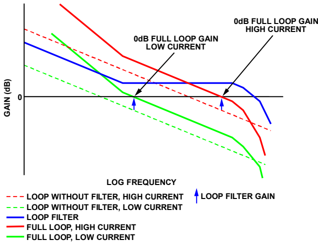
Figure 77. Gain vs. Frequency of PLL and Loop Filter
