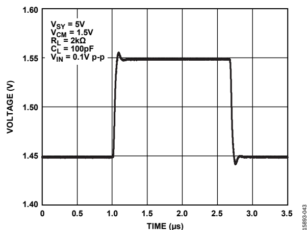
Figure 44. Small Signal Transient Response, A_V = 1 , V_{SY} = 5\text{ V}
