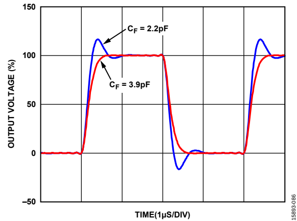
Figure 84. Pulse Response vs. C_F
