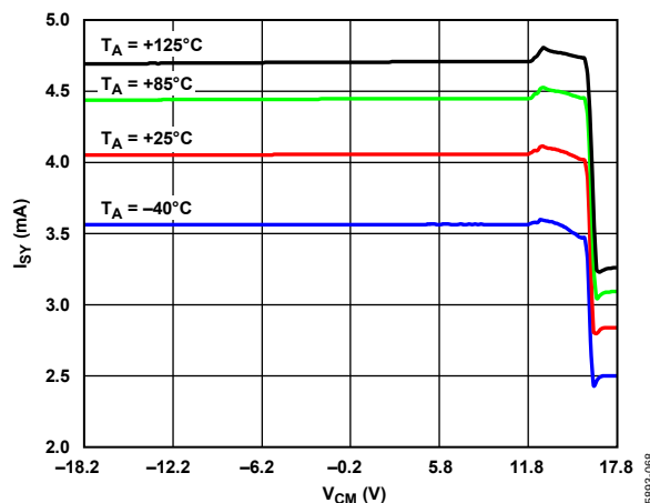
Figure 69. I_{SY} vs V_{CM} , V_{SY} = \pm 18 V
