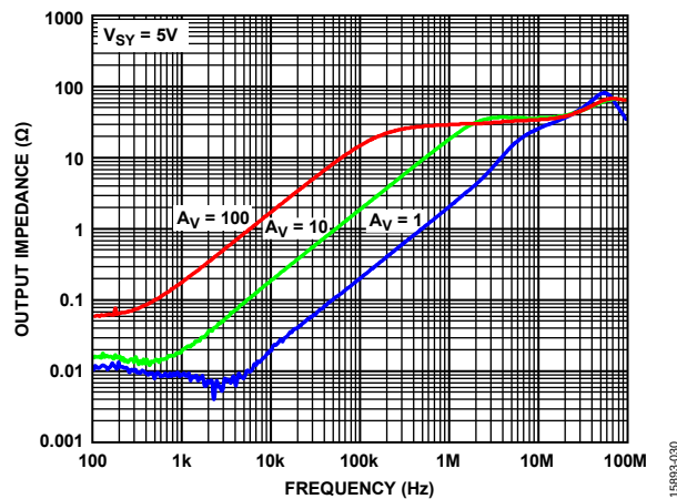
Figure 31. Z_{OUT} vs. Frequency, V_{SY} = 5V
