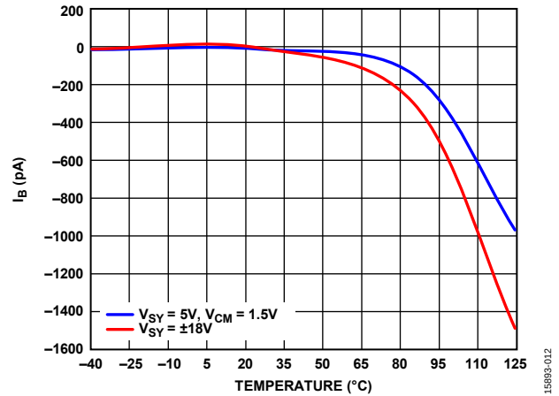
Figure 13. I_B vs. Temperature
