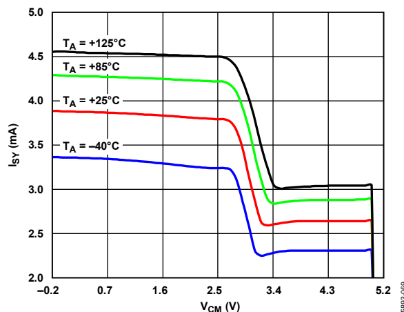
Figure 70. I_{SY} vs V_{CM} , V_{SY} = 5 V
