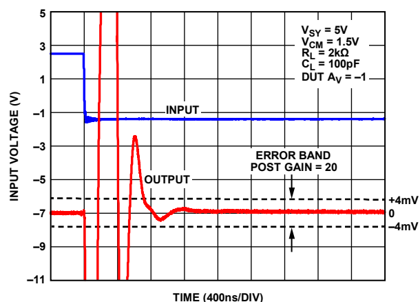
Figure 55. Negative Settling Time to 0.01%, V_{SY} = 5V
