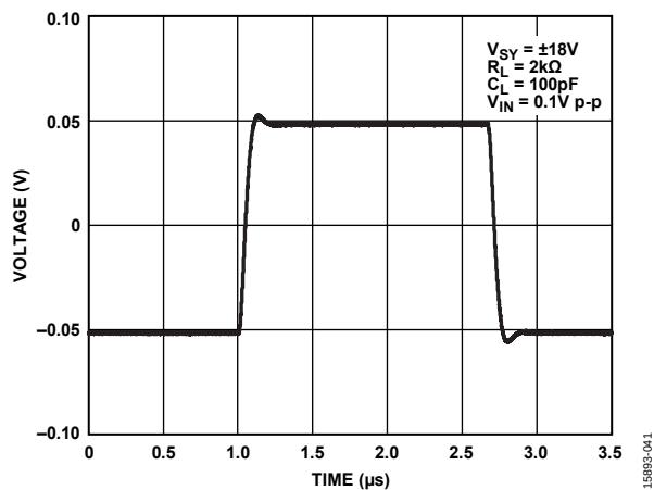
Figure 42. Small Signal Transient Response, A_V = -1 , V_{SY} = \pm 18\text{ V}
