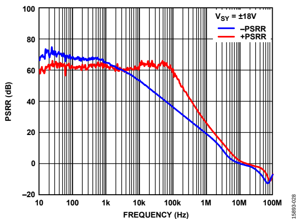
Figure 29. Power Supply Rejection Ratio (PSRR) vs. Frequency, V_{SY} = \pm 18V
