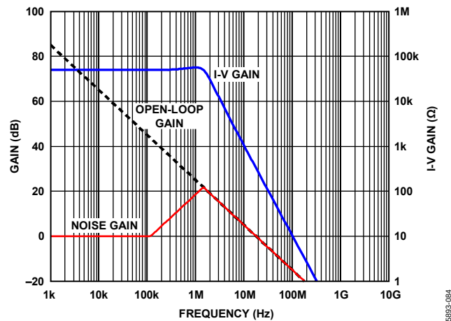
Figure 82. Compensating the TIA, C_F = 2.2 pF
