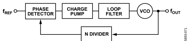
Figure 71. Basic PLL
