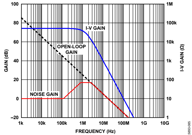
Figure 83. Compensating the TIA, C_F = 3.9 pF
