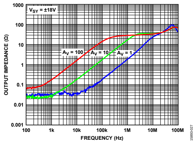
Figure 28. Output Impedance ( Z_{OUT} ) vs. Frequency, V_{SY} = \pm 18V
