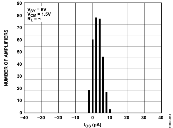
Figure 15. I_{OS} Distribution, V_{SY} = 5 V
