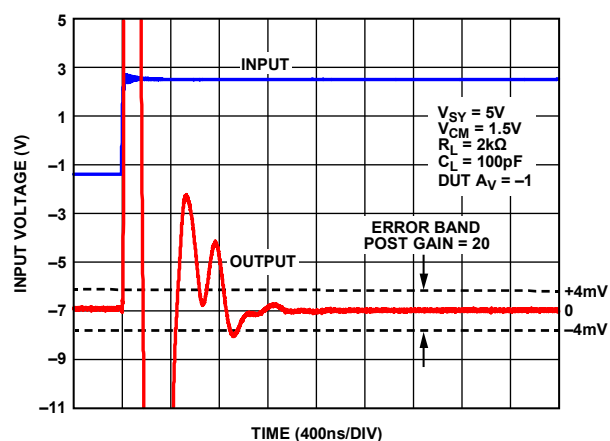
Figure 57. Positive Settling Time 0.01%, V_{SY} = 5V
