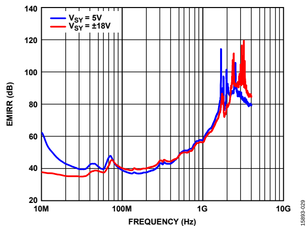
Figure 30. EMI Rejection Ratio (EMIRR) vs. Frequency
