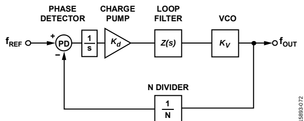
Figure 72. Basic PLL Model
