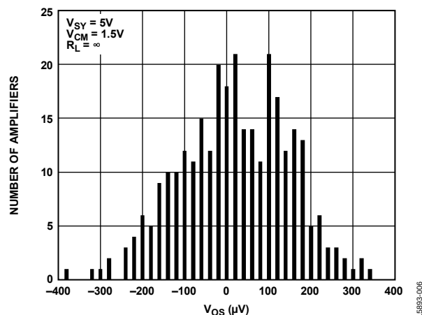
Figure 7. V_{OS} Distribution, V_{SY} = 5\text{ V}
