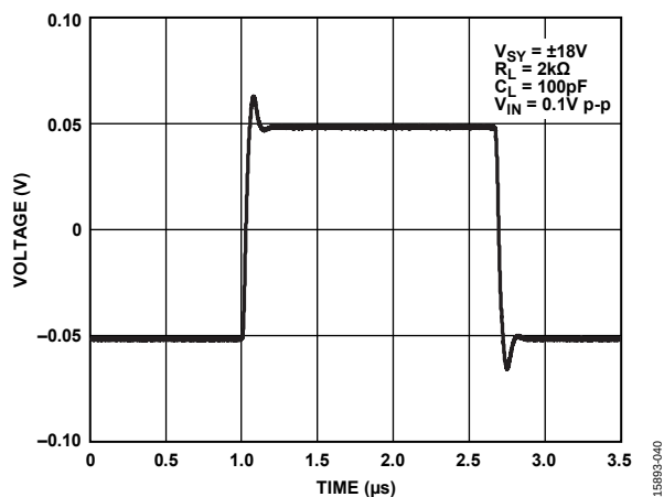
Figure 41. Small Signal Transient Response, A_V = 1 , V_{SY} = \pm 18\text{ V}
