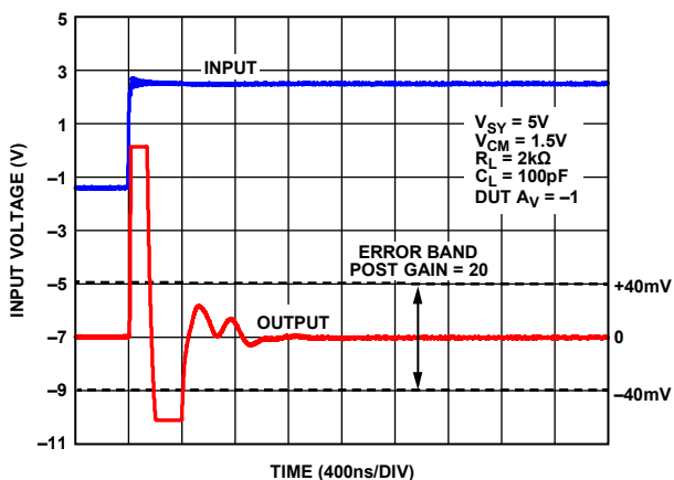
Figure 56. Positive Settling Time 0.1%, V_{SY} = 5V
