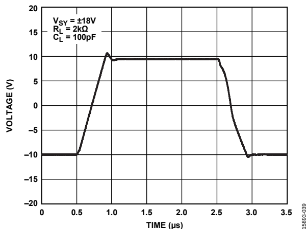
Figure 40. Large Signal Transient Response, A_V = -1 , V_{SY} = \pm 18\text{ V}
