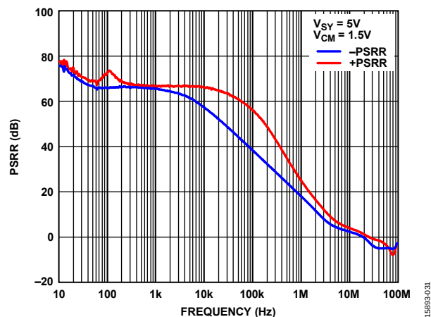
Figure 32. PSRR vs. Frequency, V_{SY} = 5V
