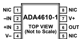
Figure 2. ADA4610-1 Pin Configuration, 8-Lead SOIC (R Suffix)
