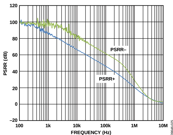
Figure 32. PSRR vs. Frequency, V_{SV} = \pm 15 V
