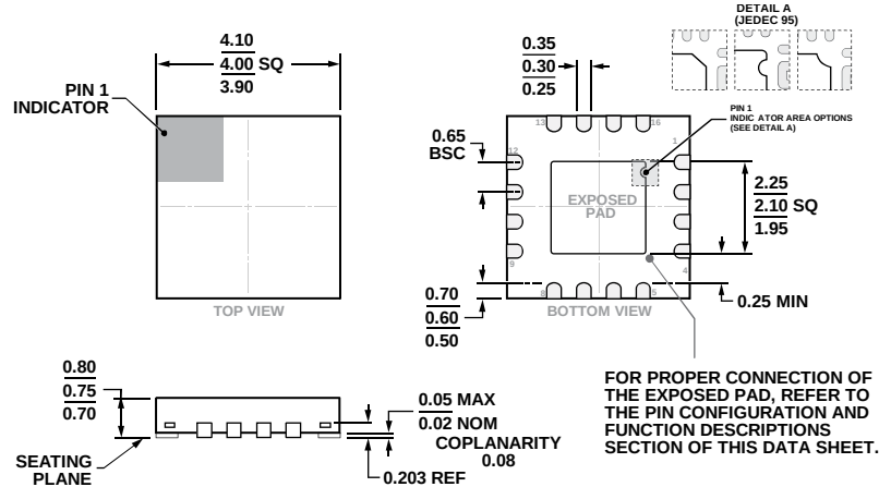
Figure 66. 16-Lead Lead Frame Chip Scale Package [LFCSP] 4 mm × 4 mm Body and 0.75 mm Package Height (CP-16-23)
