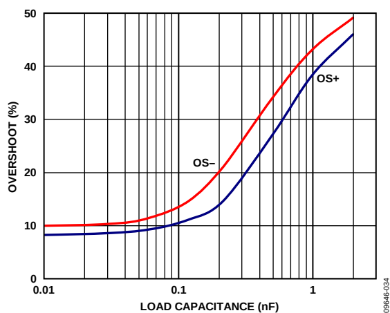
Figure 40. Overshoot vs. Load Capacitance, V_{SY} = \pm 5\text{ V} , A_V = +1 , R_L = 2\text{ k}\Omega , V_{IN} = 100\text{ mV p-p}
