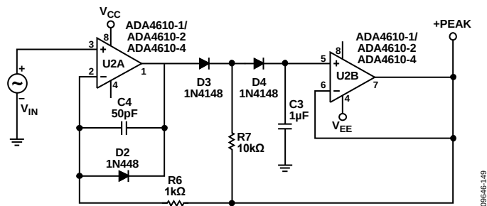
Figure 58. Positive Peak Detector
