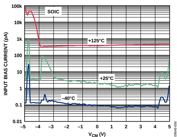
Figure 16. Input Bias Current vs. Common-Mode Input Voltage ( V_{CM} ), V_{SY} = \pm 5\text{ V} , R_L = \infty
