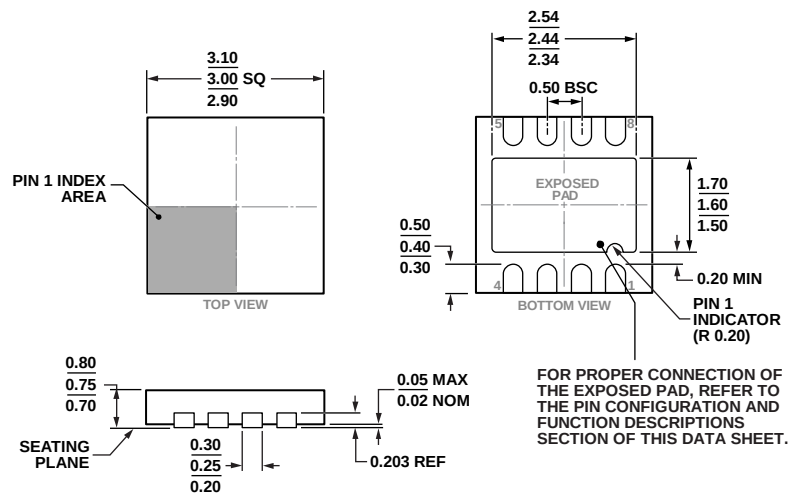
Figure 64. 8-Lead Lead Frame Chip Scale Package [LFCSP] 3 mm x 3 mm Body and 0.75 mm Package Height (CP-8-21)
