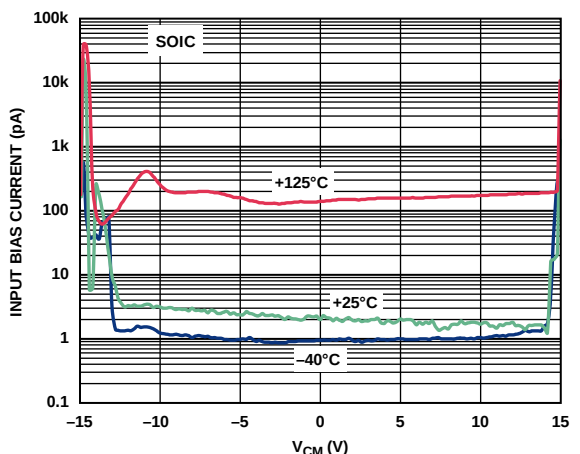
Figure 19. Input Bias Current vs. Common-Mode Input Voltage ( V_{CM} ), V_{SY} = \pm 15\text{ V} , R_L = \infty
