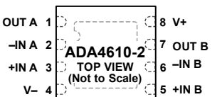
Figure 6. ADA4610-2 Pin Configuration, 8-Lead LFCSP (CP Suffix)
