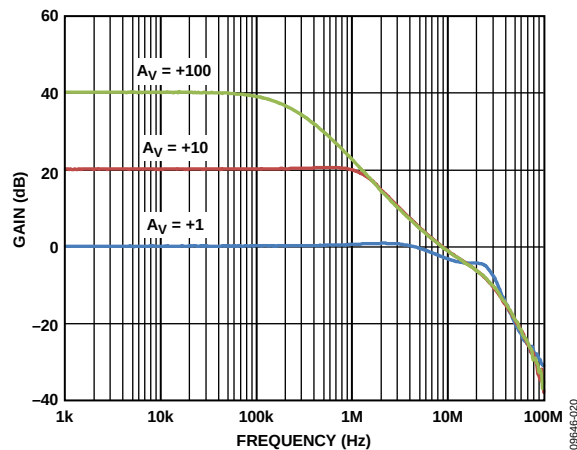
Figure 30. Closed-Loop Gain vs. Frequency, V_{SV} = \pm 15 V
