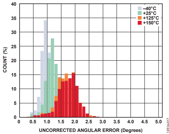
Figure 10. Uncorrected Angular Error, V_{DD} = 5.5\text{ V} , GC = Off
