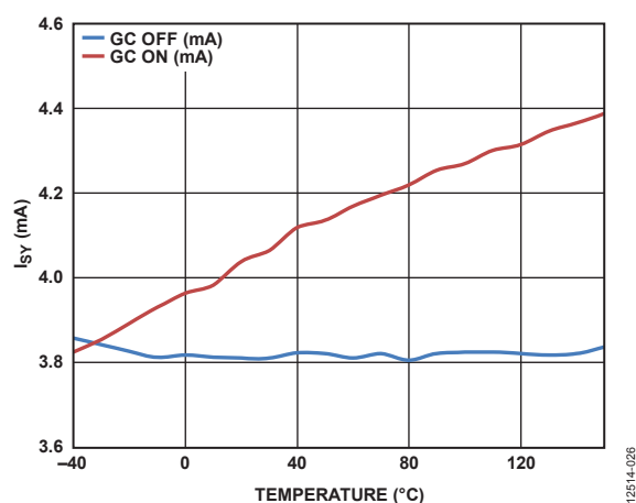
Figure 19. Supply Current ( I_{SV} ) vs. Temperature, V_{DD} = 3\text{ V}
