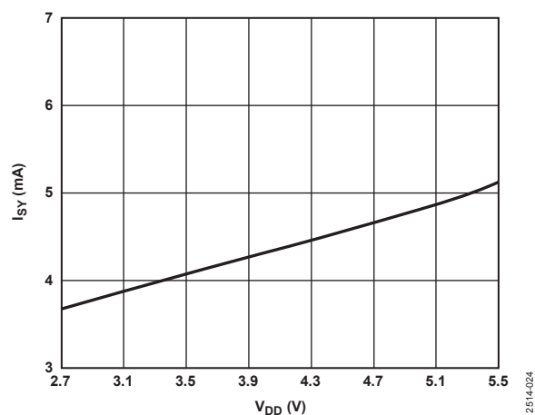
Figure 17. Supply Current ( I_{SV} ) vs. Voltage ( V_{DD} ), T = 25^\circ\text{C}
