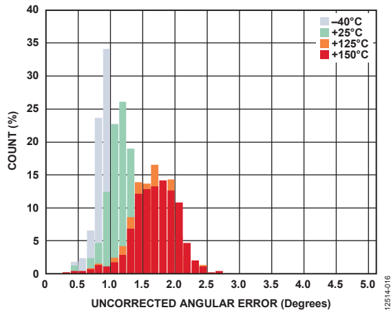
Figure 9. Uncorrected Angular Error, V_{DD} = 5.5\text{ V} , GC = On
