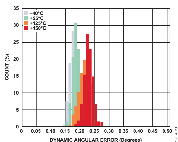
Figure 7. Dynamic Angular Error, V_{DD} = 2.7\text{ V} , GC = On
