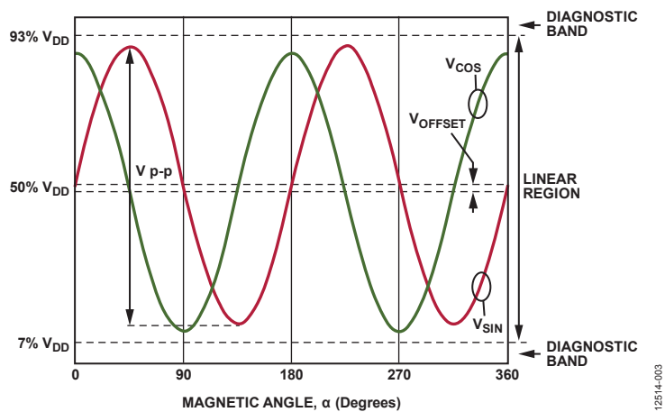
Figure 28. Typical Output Waveforms; Sine and Cosine vs. Magnetic Angle
