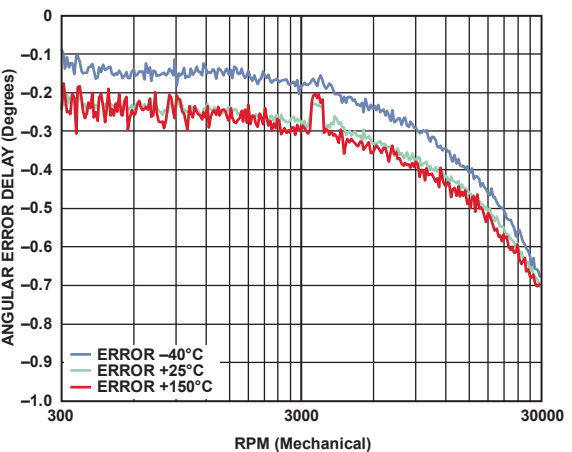
Figure 24. Angular Error Delay vs. RPM (Mechanical)
