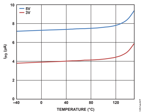
Figure 20. Power-Down Current ( I_{PD} ) vs. Temperature
