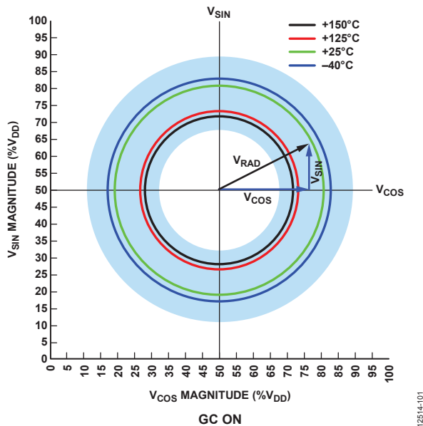
Figure 32. GC On Radius Values
