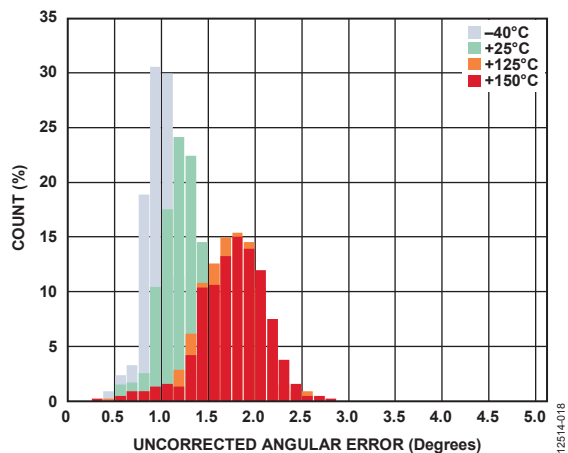
Figure 11. Uncorrected Angular Error, V_{DD} = 2.7\text{ V} , GC = On
