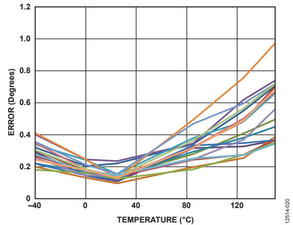
Figure 13. Single Point Calibration Angular Error, V_{DD} = 5.5\text{ V} , GC = On
