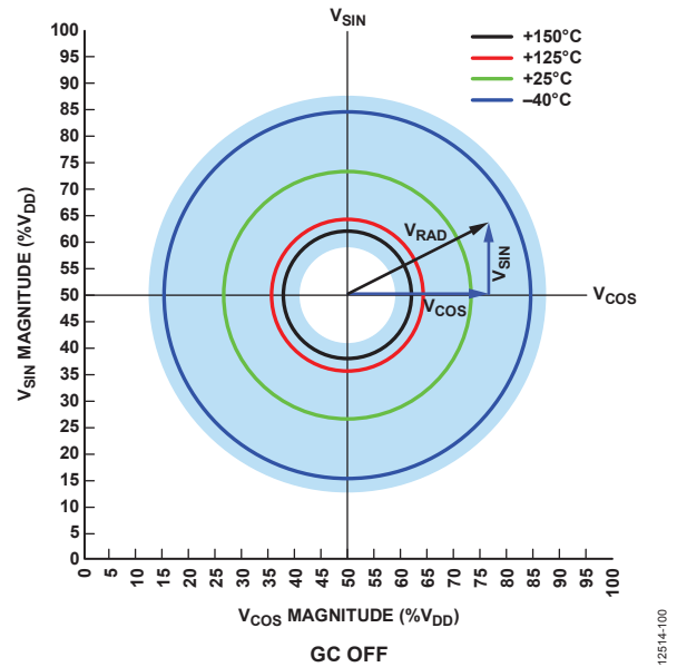
Figure 33. GC Off Radius Values
