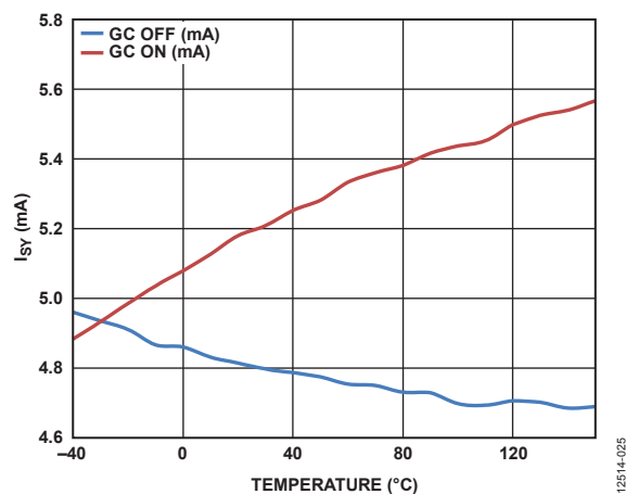
Figure 18. Supply Current ( I_{SV} ) vs. Temperature, V_{DD} = 5\text{ V}
