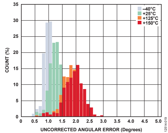
Figure 12. Uncorrected Angular Error, V_{DD} = 2.7\text{ V} , GC = Off
