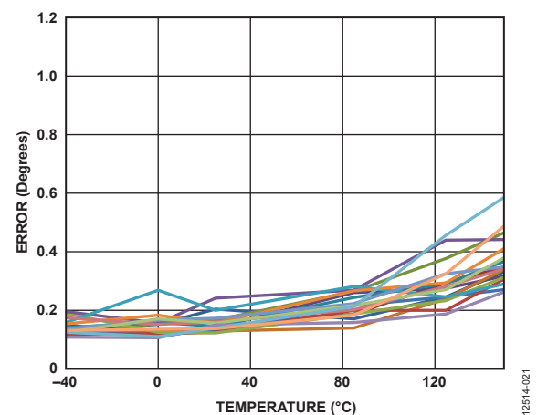
Figure 14. Single Point Calibration Angular Error, V_{DD} = 5.5\text{ V} , GC = Off
