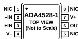
Figure 1. ADA4528-1 Pin Configuration, 8-Lead MSOP
