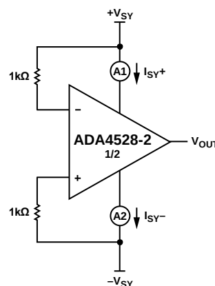
Figure 70. Comparator A
