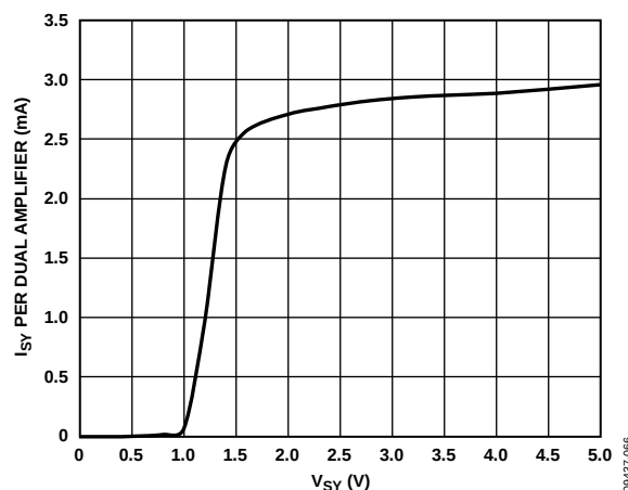
Figure 69. Supply Current vs. Supply Voltage (Voltage Follower)
