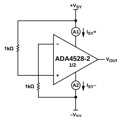
Figure 71. Comparator B
