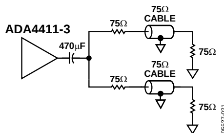
Figure 23. Driving Two AC-Coupled Loads with One Common Coupling Capacitor
