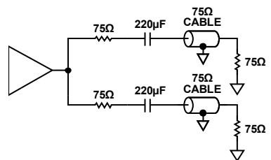
Figure 25. Driving Two AC-Coupled Loads with Two Coupling Capacitors
