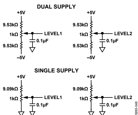
Figure 23. Generating Fully Adjustable Output Offsets
