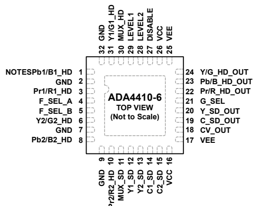
Figure 3. 32-Lead LFCSP Pin Configuration, Top View
