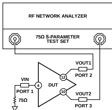
Figure 19. Test Circuit for S_{23} , S_{32} Measurements
