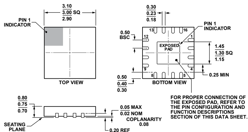
Figure 20. 16-Lead Lead Frame Chip Scale Package [LFCSP] 3 mm × 3 mm Body and 0.75 mm Package Height (CP-16-21)
