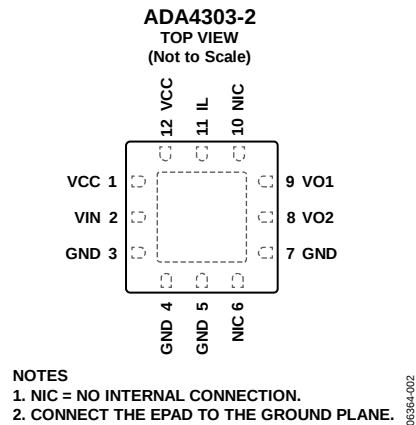
Figure 4. Pin Configuration
