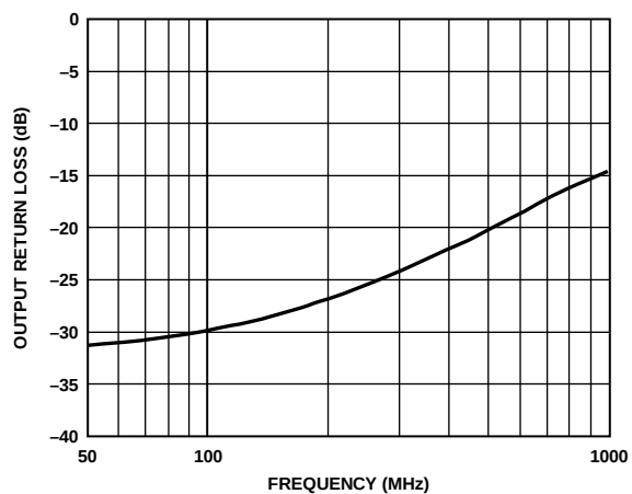
Figure 15. Output Return Loss (S22) vs. Frequency
