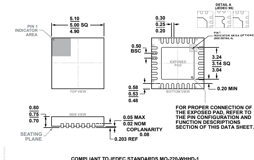
Figure 111. 28-Lead Lead Frame Chip Scale Package [LFCSFP] 5 mm × 5 mm Body and 0.75 mm Package Height (CP-28-10)
