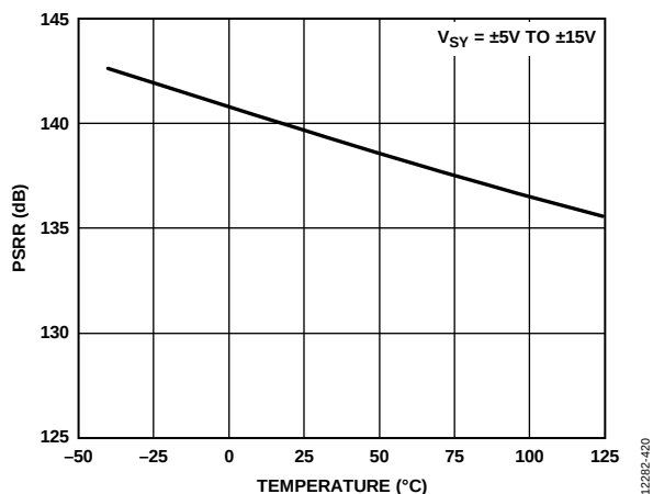
Figure 53. Power Supply Rejection Ratio (PSRR) vs. Temperature, V_{SV} = \pm 5V to \pm 15V
