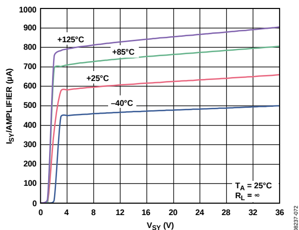
Figure 103. Supply Current ( I_{SV} ) per Amplifier vs. Supply Voltage ( V_{SV} ) for Various Temperatures
