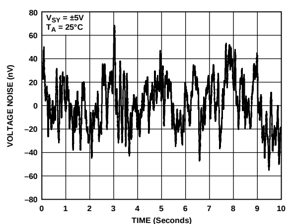
Figure 64. Voltage Noise, 0.1 Hz to 10 Hz
