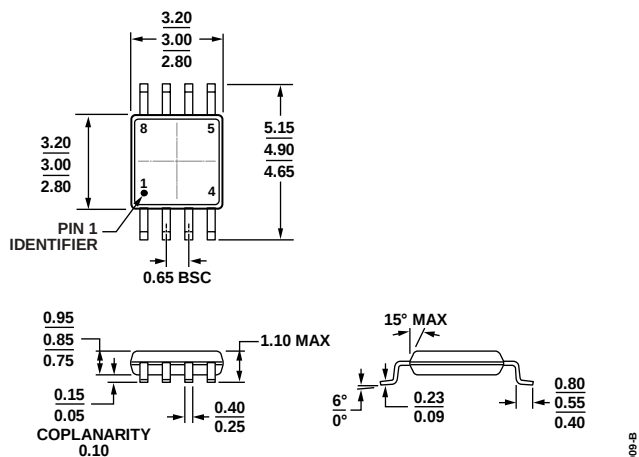
Figure 117. 8-Lead Mini Small Outline Package [MSOP] (RM-8)
