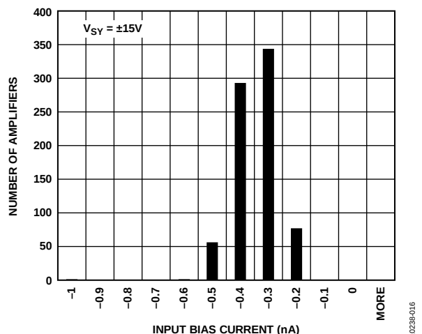
Figure 27. Input Bias Current, V_S = \pm 15V
