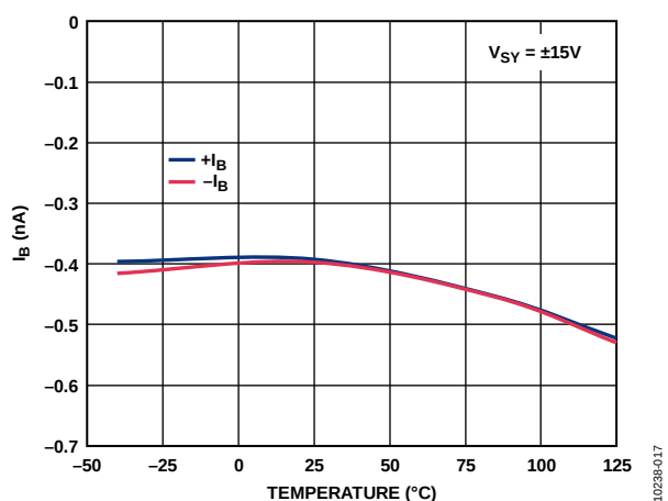
Figure 28. Input Bias Current ( I_B ) vs. Temperature, V_S = \pm 15V
