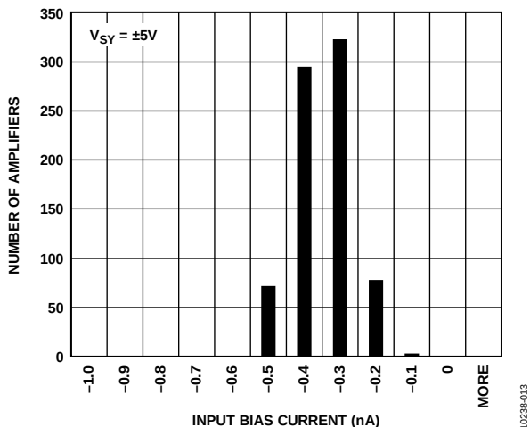
Figure 24. Input Bias Current, V_S = \pm 5V
