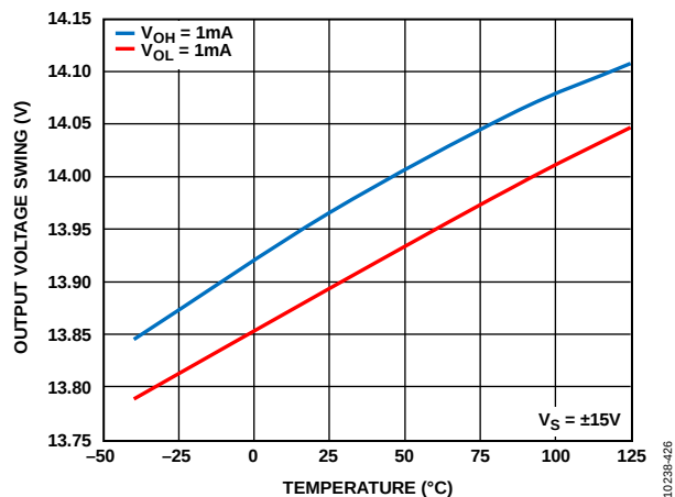
Figure 26. Output Voltage Swing vs. Temperature, V_S = \pm 15V
