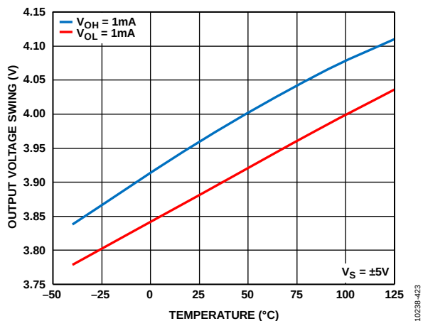
Figure 23. Output Voltage Swing vs. Temperature, V_S = \pm 5V
