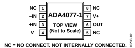
Figure 1. ADA4077-1, 8-Lead SOIC (and 8-Lead MSOP)
