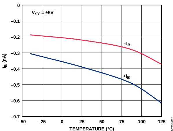
Figure 25. Input Bias Current ( I_B ) vs. Temperature, V_S = \pm 5V
