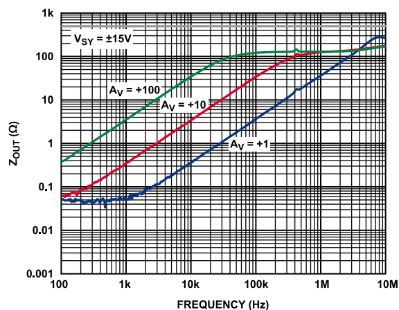
Figure 44. Output Impedance ( Z_{OUT} ) vs. Frequency, V_{SY} = \pm 15V
