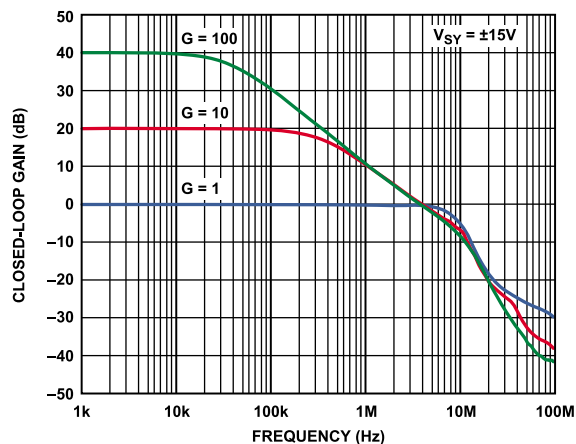
Figure 43. Closed-Loop Gain vs. Frequency, V_{SY} = \pm 15V
