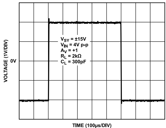
Figure 45. Large Signal Transient Response, V_{SY} = \pm 15V
