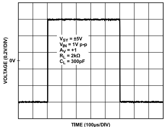
Figure 42. Large Signal Transient Response, V_{SY} = \pm 5V
