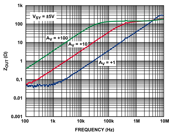
Figure 41. Output Impedance ( Z_{OUT} ) vs. Frequency, V_{SY} = \pm 5V
