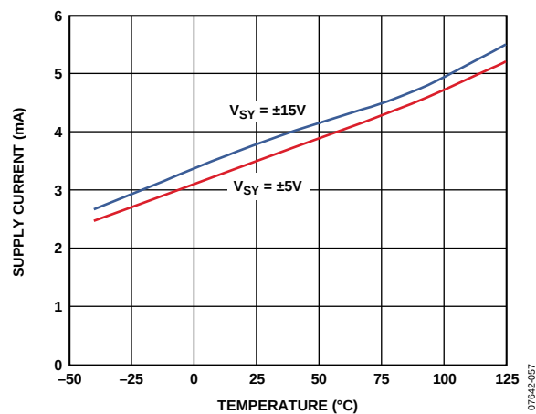
Figure 54. Supply Current vs. Temperature
