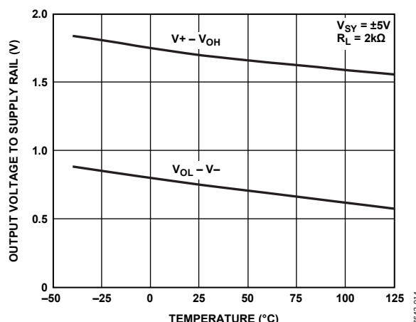
Figure 20. Output Voltage to Supply Rail vs. Temperature
