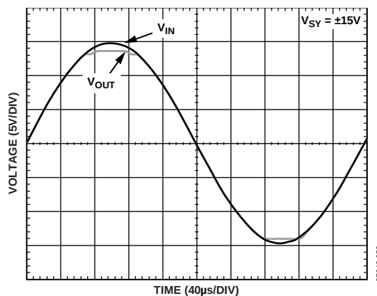
Figure 65. No Phase Reversal
