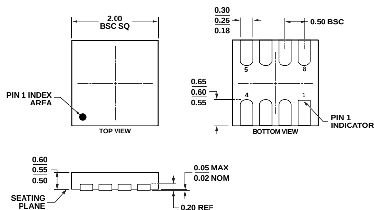
Figure 72. 8-Lead Lead Frame Chip Scale Package [LFCSF_WD] 2 mm x 2 mm Body, Very Very Thin, Dual Lead (CP-8-6)
