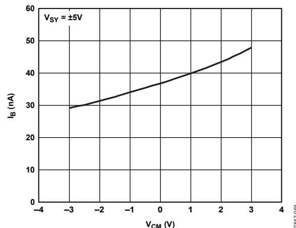
Figure 18. Input Bias Current vs. Input Common-Mode Voltage
