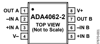
Figure 1. 8-Lead Narrow-Body SOIC and 8-Lead MSOP
