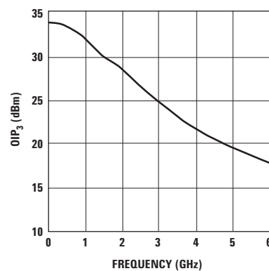
Figure 5. OIP_3 vs. Frequency at I_d = 60 mA.
