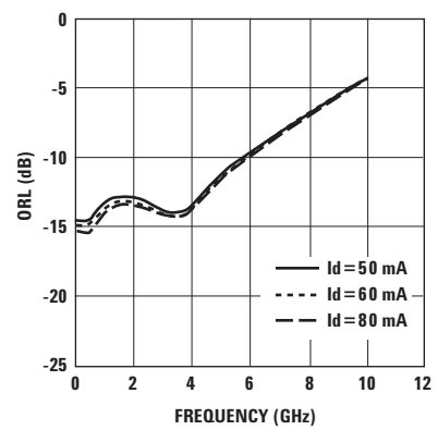
Figure 17. Output Return Loss vs. I_d and Frequency.
