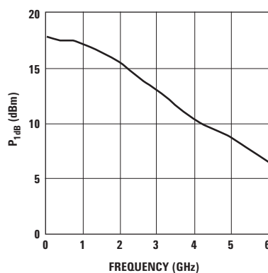
Figure 4. P_{1dB} vs. Frequency at I_d = 60 mA.
